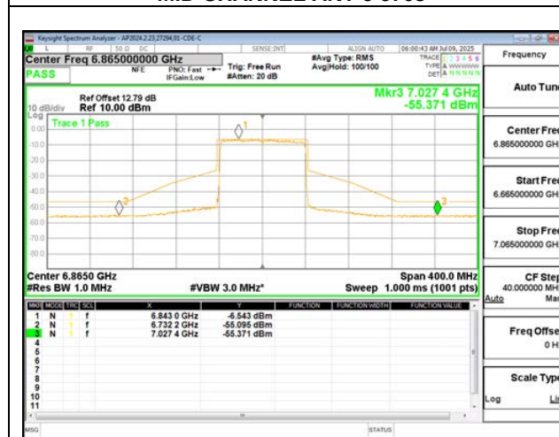
STRADDLE CHANNEL ANT 6 6865
