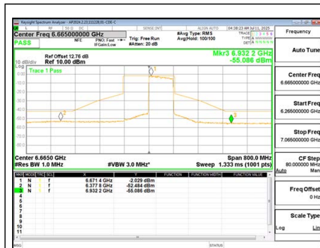
MID CHANNEL ANT 6 6665
