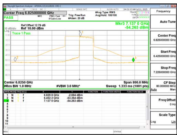
STRADDLE CHANNEL ANT 6 6825
