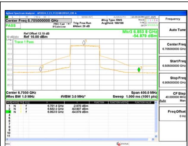
MID CHANNEL ANT 5 6705
