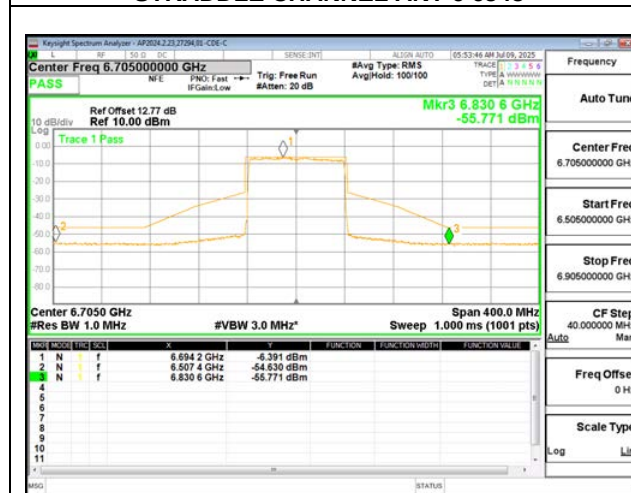
MID CHANNEL ANT 6 6705
