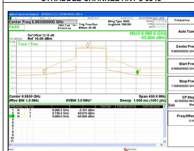
STRADDLE CHANNEL ANT 5 6865
