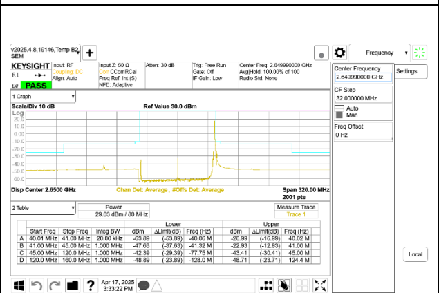
5G NR n41 80MHz BPSK High Channel RB1-216
