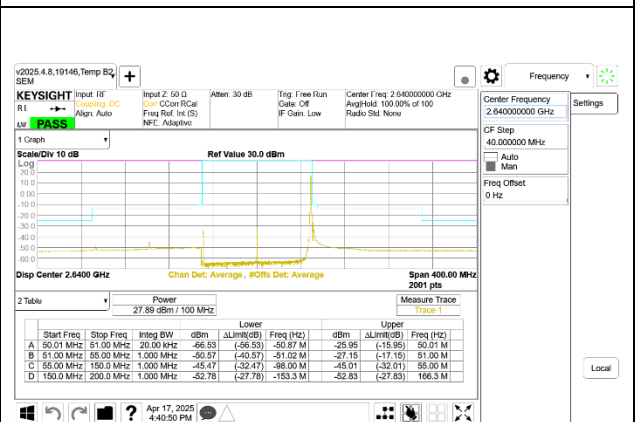
5G NR n41 100MHz BPSK High Channel RB1-272
