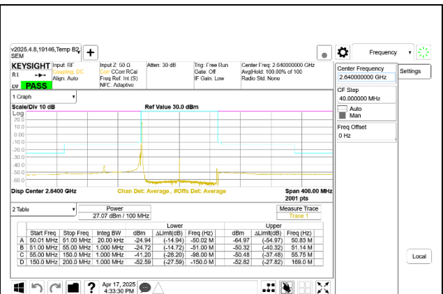
5G NR n41 100MHz BPSK High Channel RB1-0
