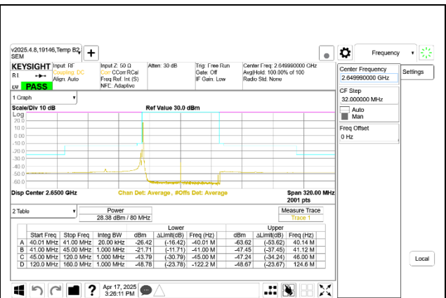
5G NR n41 80MHz BPSK High Channel RB1-0
