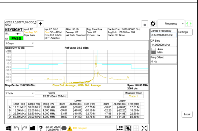
5G NR n41 35MHz BPSK High Channel RB1-91
