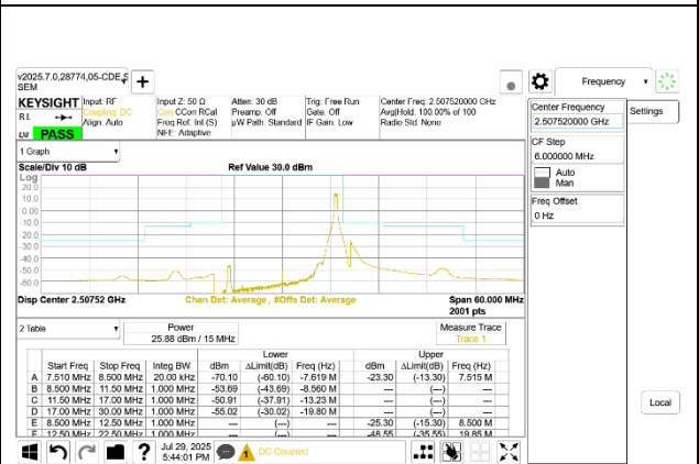
5G NR n41 15MHz BPSK Low Channel RB1-37
