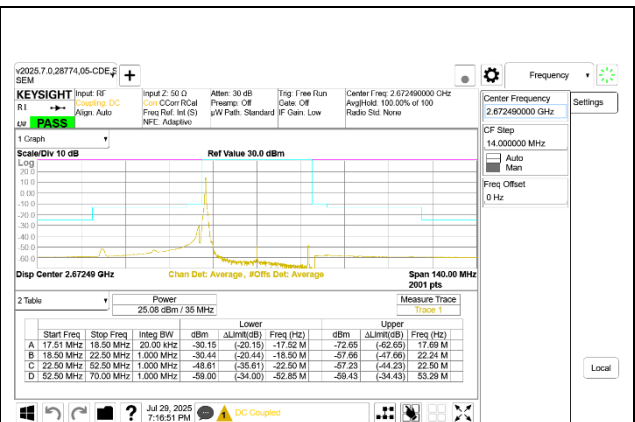
5G NR n41 35MHz BPSK High Channel RB1-0
