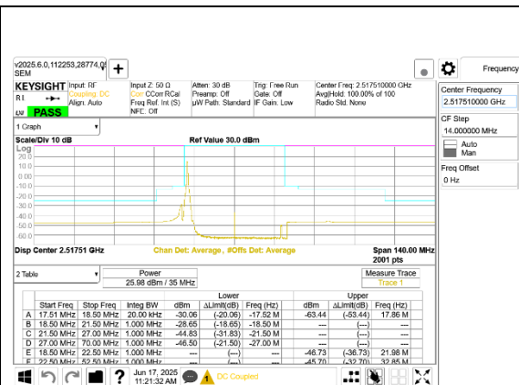
5G NR n41 35MHz BPSK Low Channel RB1-0
