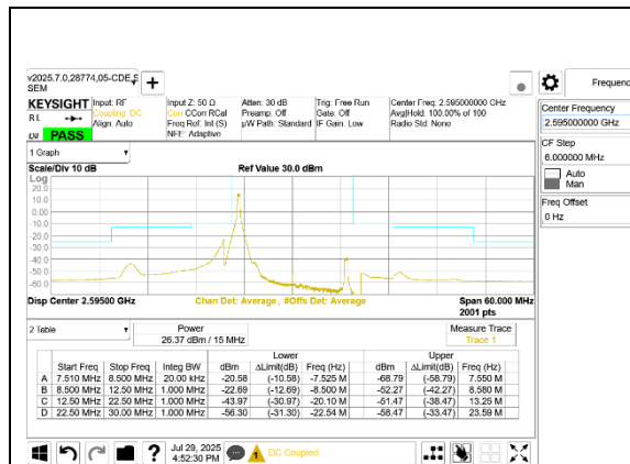
5G NR n41 15MHz BPSK Middle Channel RB1-0
