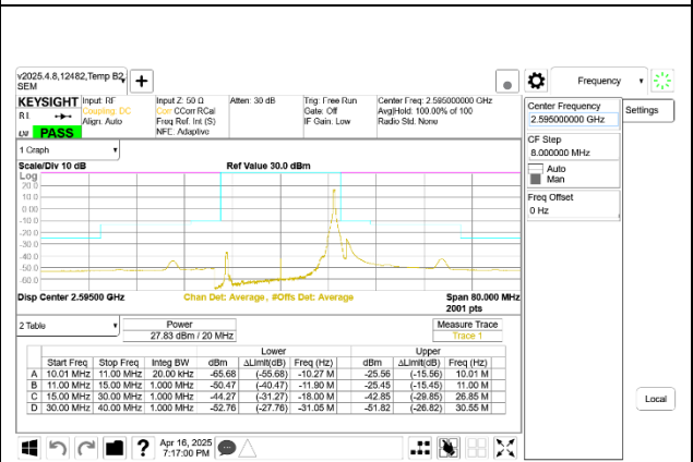
5G NR n41 20MHz BPSK Middle Channel RB1-50
