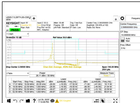
5G NR n41 35MHz BPSK Middle Channel RB1-0
