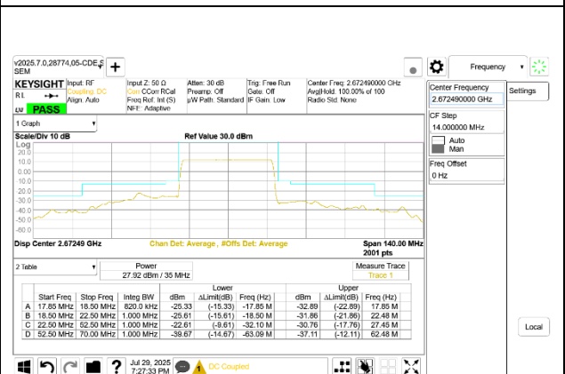
5G NR n41 35MHz BPSK High Channel RB90-0
