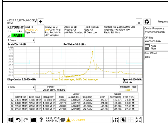
5G NR n41 15MHz BPSK Middle Channel RB1-37
