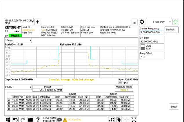
5G NR n41 30MHz BPSK Middle Channel RB75-0
