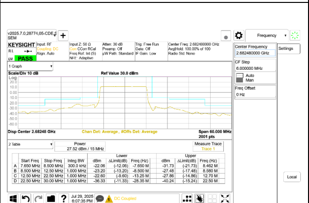
5G NR n41 15MHz BPSK High Channel RB36-0
