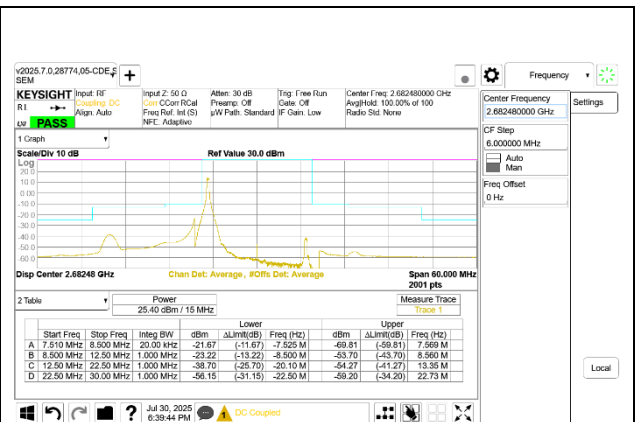
5G NR n41 15MHz BPSK High Channel RB1-0
