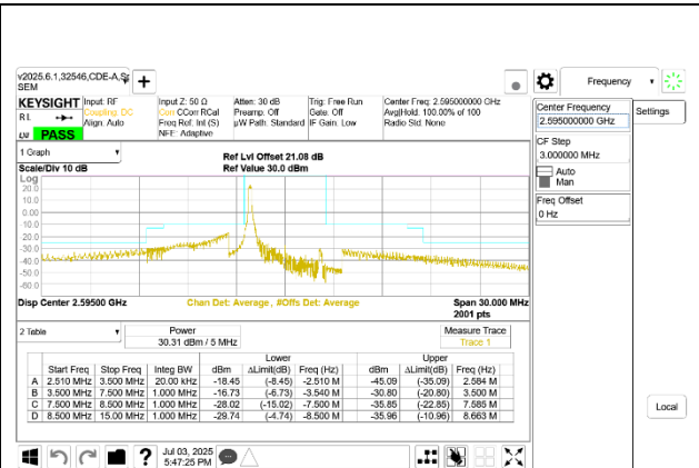
LTE B41 5MHz QPSK Middle Channel RB1-0
