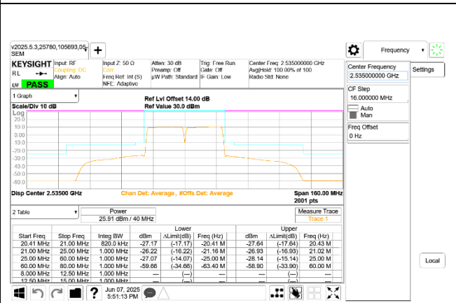
ULCA LTE B7 20MHz + 20MHz 16QAM Mid Ch RB100-0 + RB100-0
