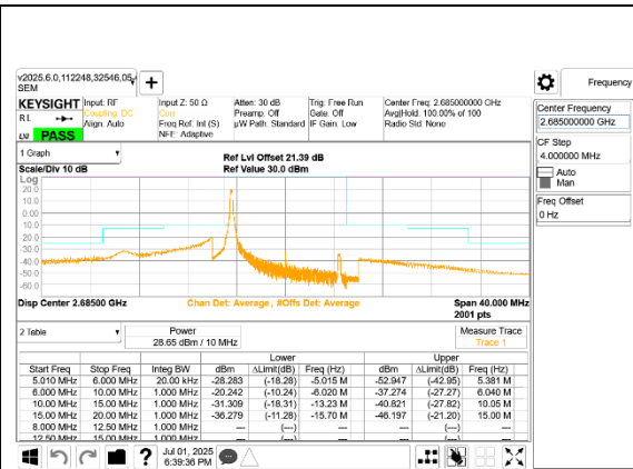
LTE B41 10MHz QPSK High Channel RB1-0
