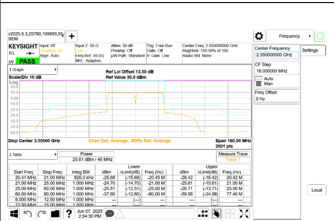
ULCA LTE B7 20MHz + 20MHz 16QAM High Ch RB100-0 + RB100-0
