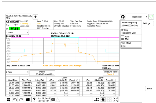
ULCA LTE B7 20MHz + 20MHz QPSK High Ch RB100-0 + RB100-0
