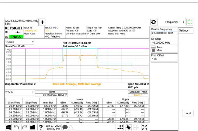
ULCA LTE B7 20MHz + 20MHz 16QAM Low Ch RB100-0 + RB100-0
