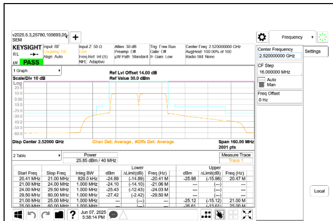
ULCA LTE B7 20MHz + 20MHz QPSK Low Ch RB100-0 + RB100-0
