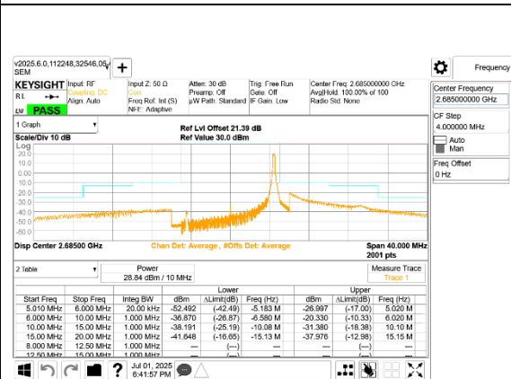
LTE B41 10MHz QPSK High Channel RB1-49
