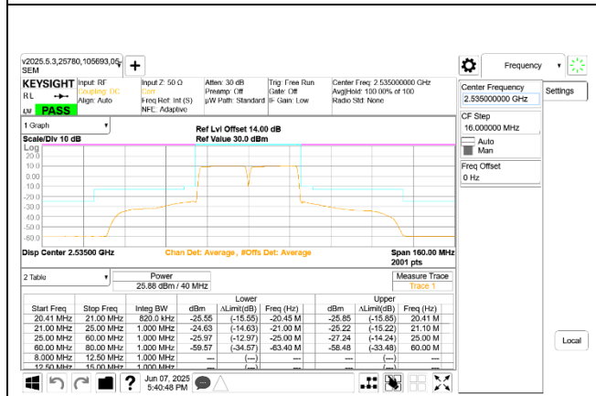
ULCA LTE B7 20MHz + 20MHz QPSK Mid Ch RB100-0 + RB100-0
