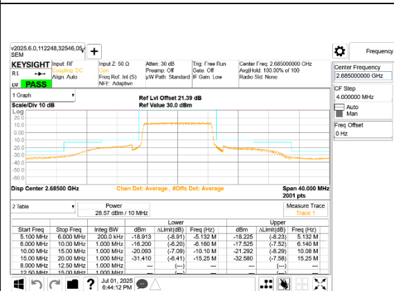
LTE B41 10MHz QPSK High Channel RB50-0
