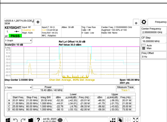
ULCA LTE B7 20MHz + 20MHz 16QAM High Ch RB1-0 + RB1-99
