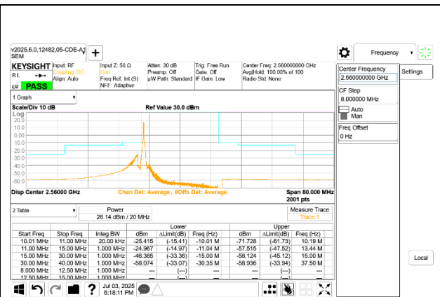
5G NR n7 20MHz BPSK High Channel RB1-0
