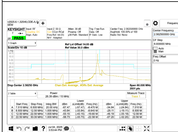
LTE B7 15MHz QPSK High Channel RB1-74
