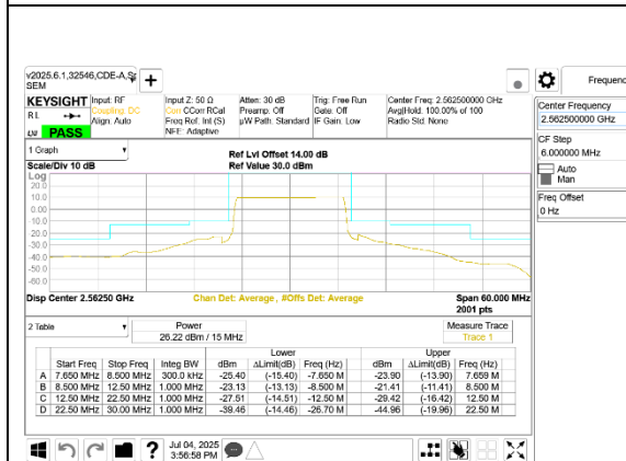
LTE B7 15MHz QPSK High Channel RB75-0
