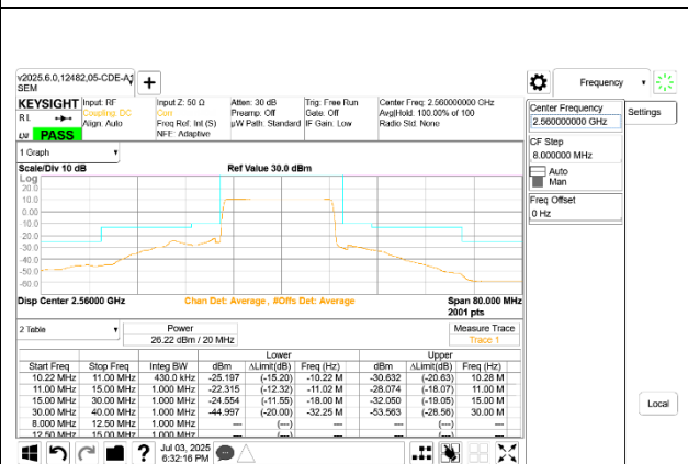
5G NR n7 20MHz BPSK High Channel RB100-0
