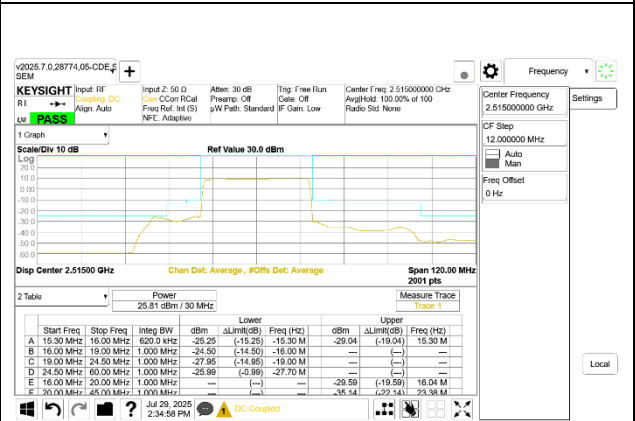
5G NR n7 30MHz BPSK Low Channel RB160-0
