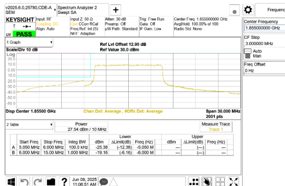
LTE B25 10MHz QPSK Low Channel RB50-0
