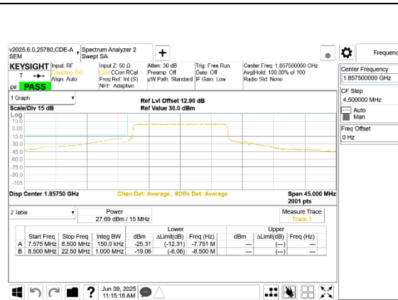
LTE B25 15MHz QPSK Low Channel RB75-0
