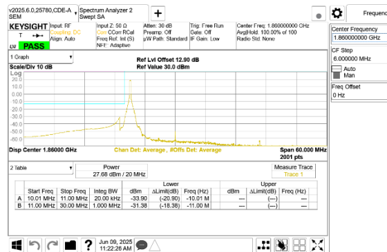
LTE B25 20MHz QPSK Low Channel RB1-0
