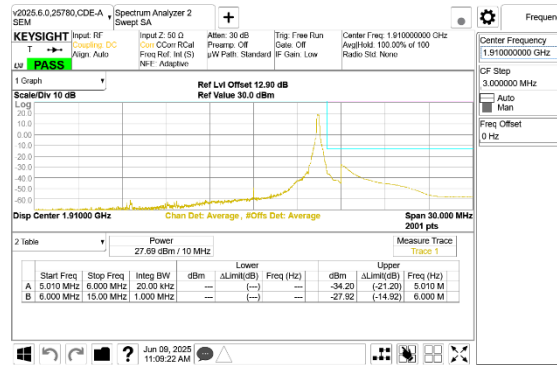
LTE B25 10MHz QPSK High Channel RB1-49
