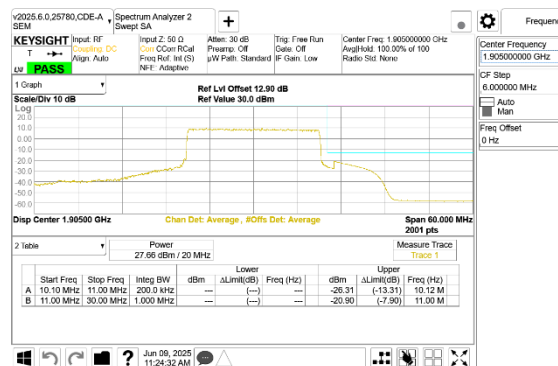
LTE B25 20MHz QPSK High Channel RB100-0
