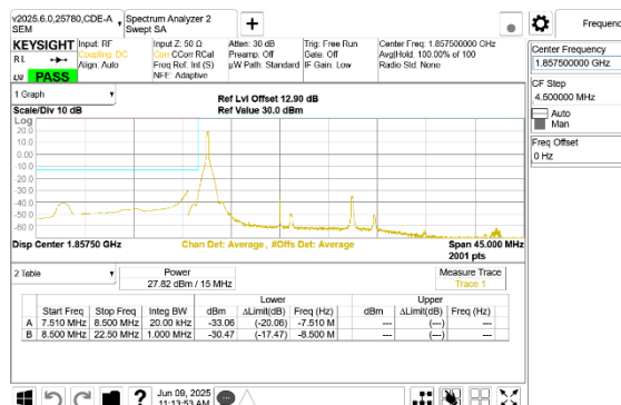
LTE B25 15MHz QPSK Low Channel RB1-0
