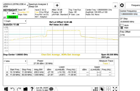
LTE B25 20MHz QPSK Low Channel RB100-0
