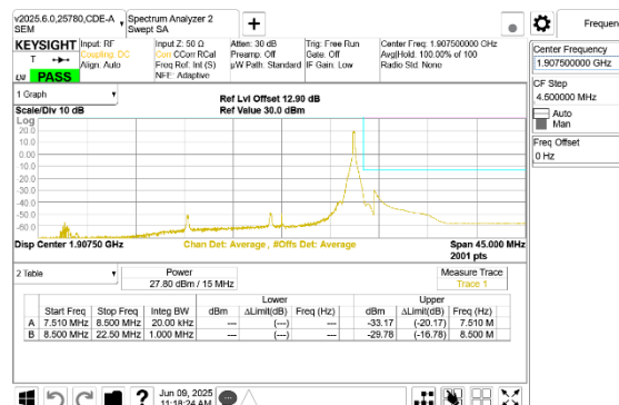
LTE B25 15MHz QPSK High Channel RB1-74
