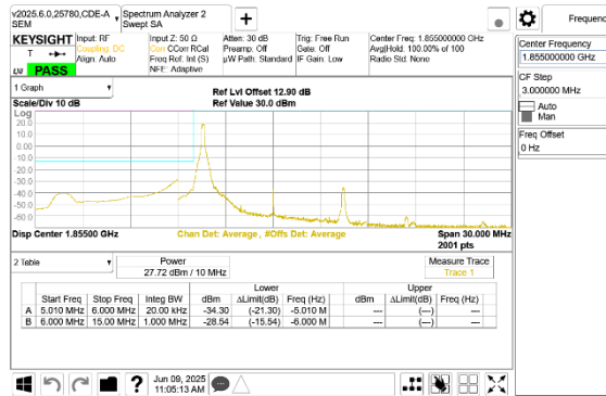
LTE B25 10MHz QPSK Low Channel RB1-0
