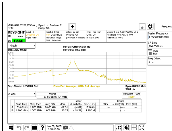
LTE B25 1.4MHz QPSK Low Channel RB1-0
