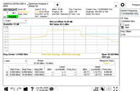
LTE B25 10MHz QPSK High Channel RB50-0
