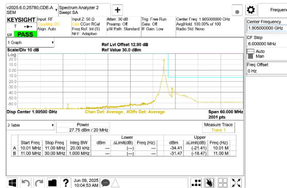
LTE B25 20MHz QPSK High Channel RB1-99
