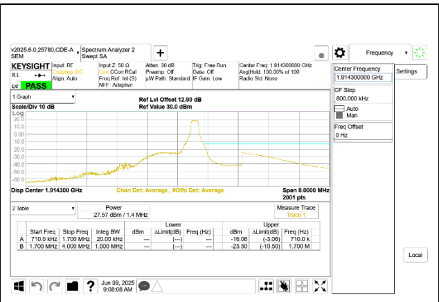
LTE B25 1.4MHz QPSK High Channel RB1-5
