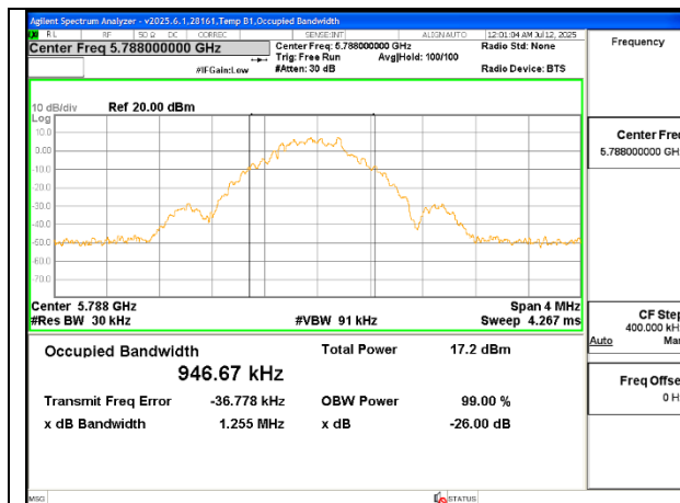
Mid Channel (UNII-3 LE1M) – Ant 6
