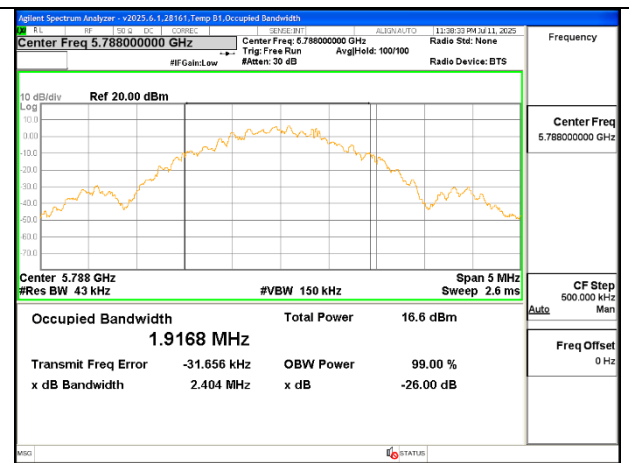
Mid Channel (UNII-3 BLE2M) – Ant 5
