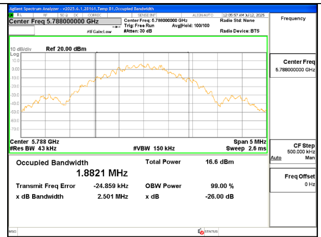
Mid Channel (UNII-3 LE2M) – Ant 5
