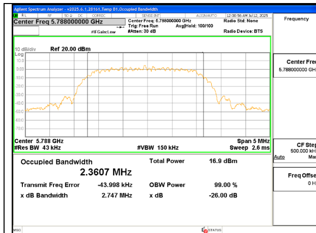
Mid Channel (UNII-3 HDT2) – Ant 6
