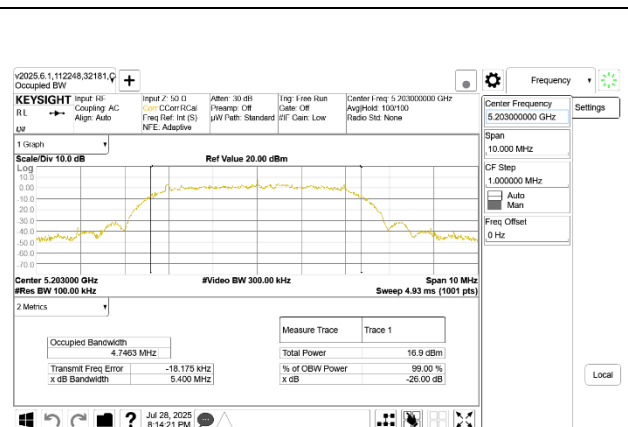
Mid Channel (UNII-1 HDRPM8) – Ant 5
