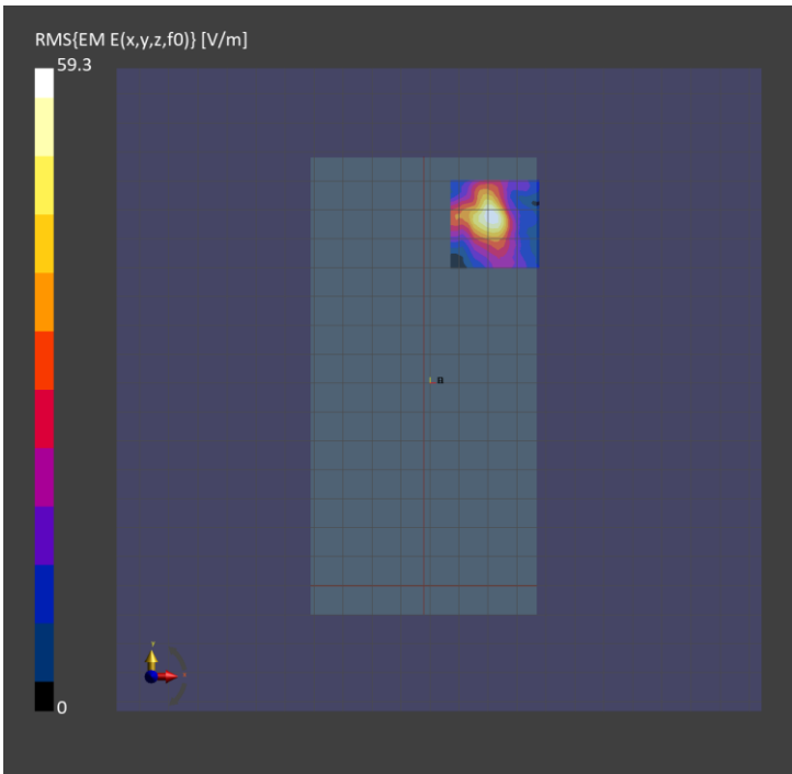
Figure 6-1: Band n258, Beam ID 276, point PD and 4cm² PD, Top
