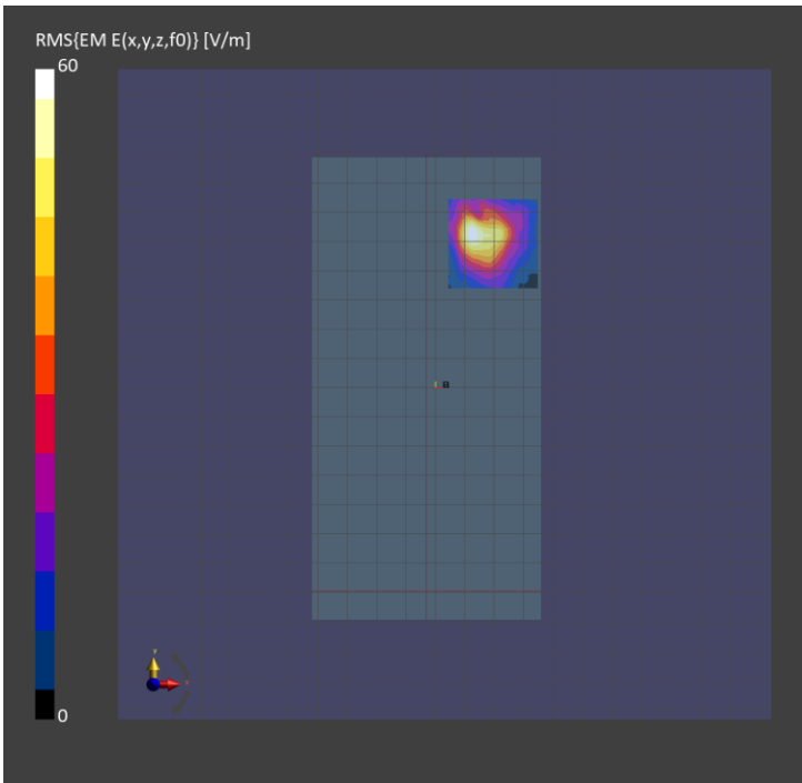
Figure 6-2: Band n260, Beam ID 13, point PD and 4cm² PD, Back
