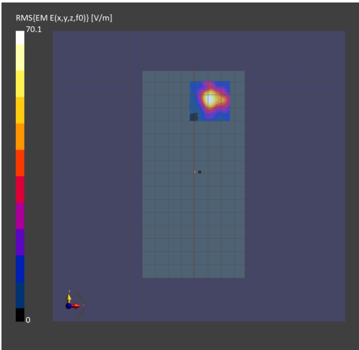
Figure 6-3: Band n261, Beam ID 269, point PD and 4cm² PD, Back
