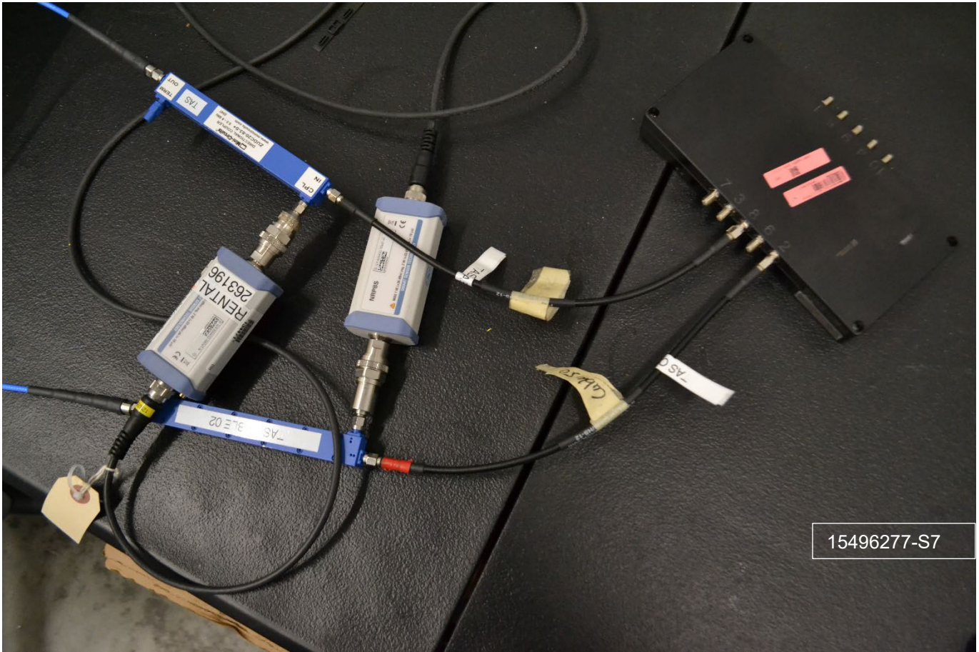
Figure D-2 CMW & UXM Conducted power test measurement setup dual port
