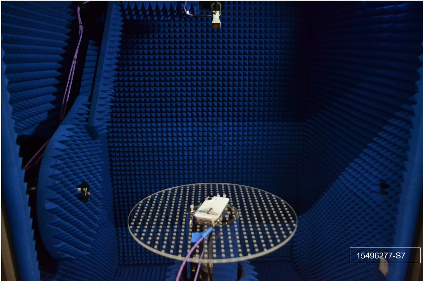
Figure D-3 Radiated power mmW test measurement setup
