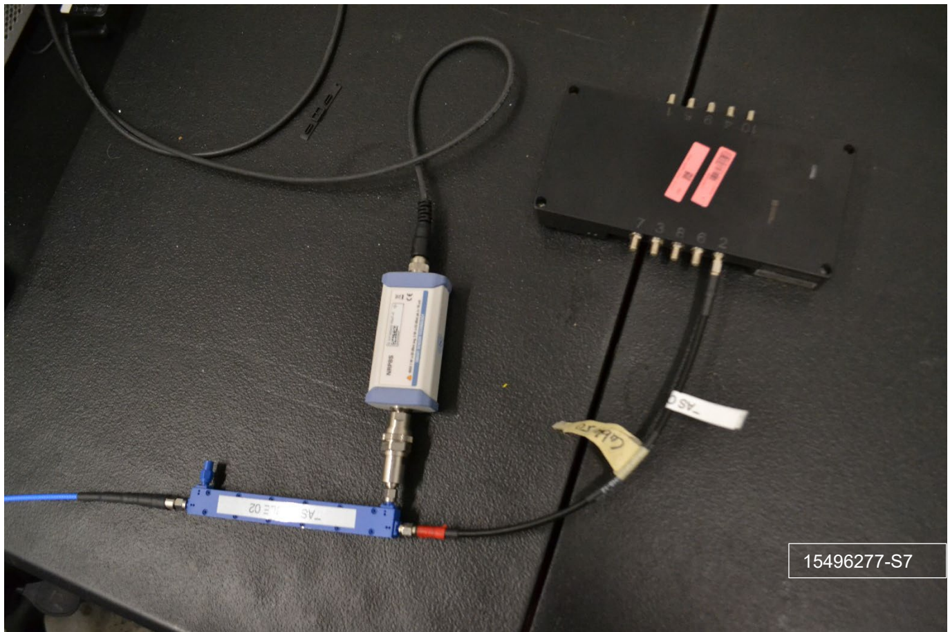
Figure D-1 CMW Conducted Power Test Measurement setup single port
