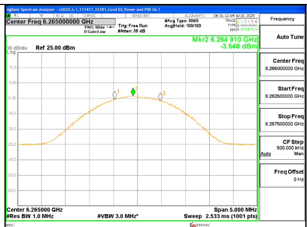
Mid Channel (UNII-5 LE1M) – Ant 5
