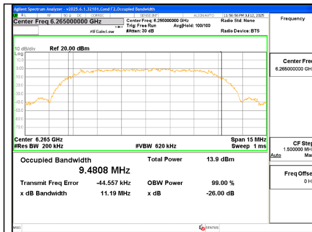
Mid Channel (UNII-5 HDRPL8) – Ant 6
