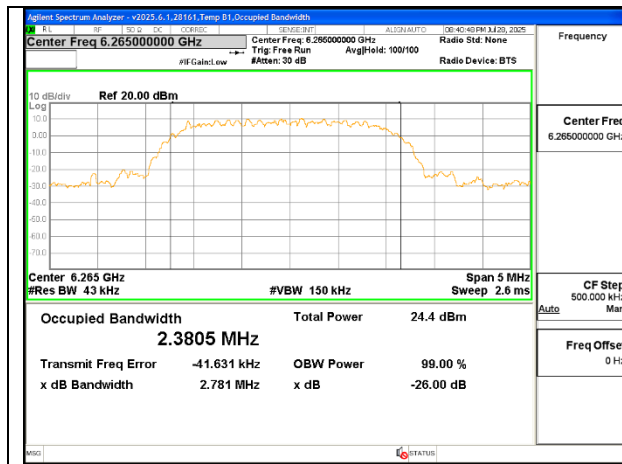
Mid Channel (UNII-5 HDT4) – Ant 6
