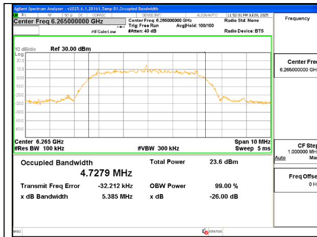
Mid Channel (UNII-5 HDRPM12) – Ant 6
