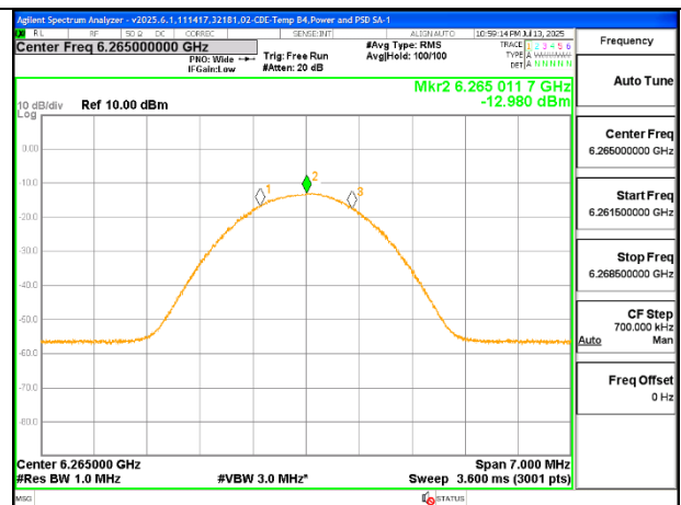
Mid Channel (UNII-5 BDR) – Ant 5
