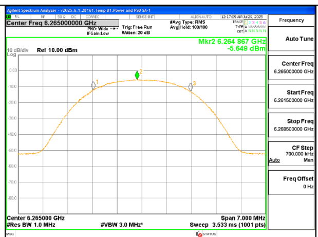
Mid Channel (UNII-5 HDT4) – Ant 5
