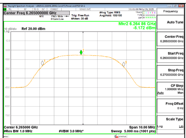
Mid Channel (UNII-5 XHDRPM8) – Ant 5
