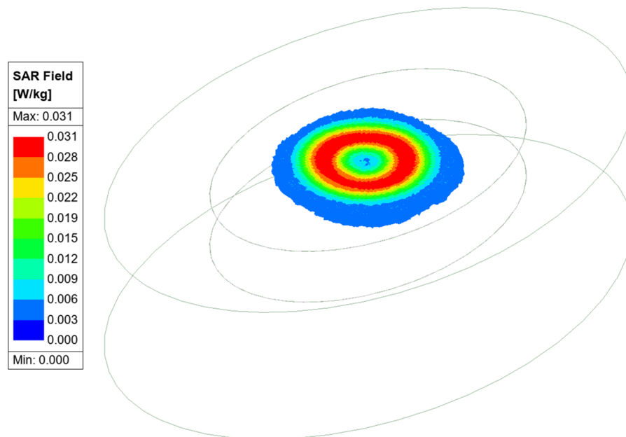
(a) Average SAR plot for direct exposure Case
