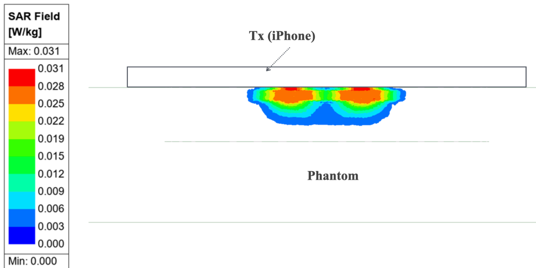
(b) Side view of average SAR plot for direct exposure Case
