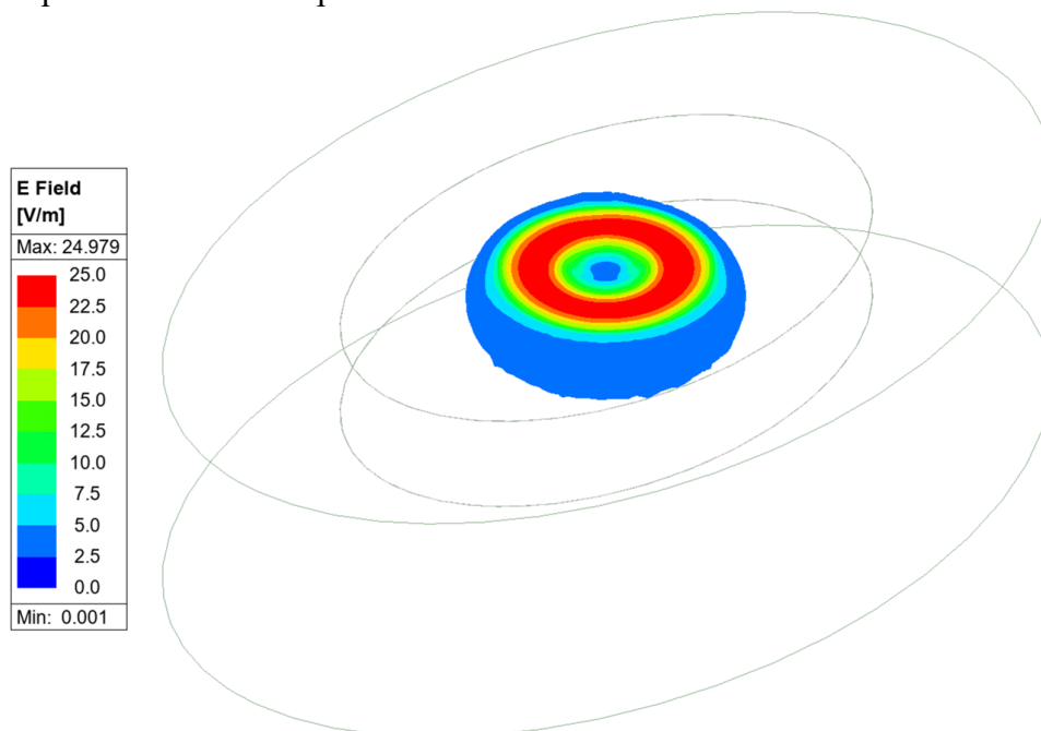
Figure 7: Peak E-field distribution inside phantom for direct exposure case
