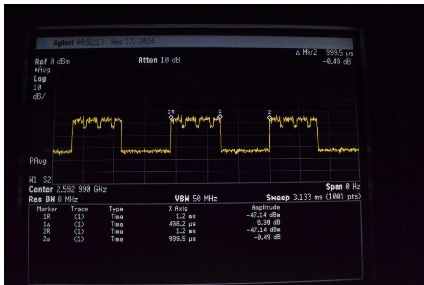
Figure 4: 5G NR TDD Power Class 2, 50% RB
