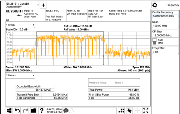
80MHz – 484+242T – Mid Channel – Puncture Pattern 8 – (UNII-2c) – Ant 5
