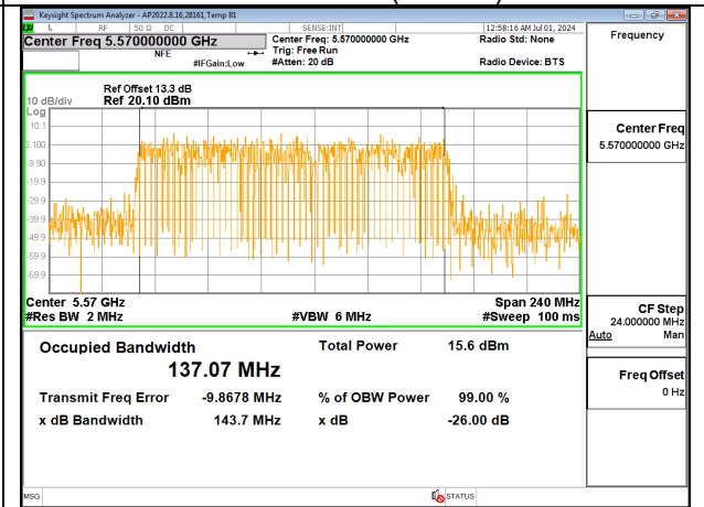
160MHz – 996+484+242T - Mid Channel – Puncture Pattern 128– (UNII-2c) – Ant 5
