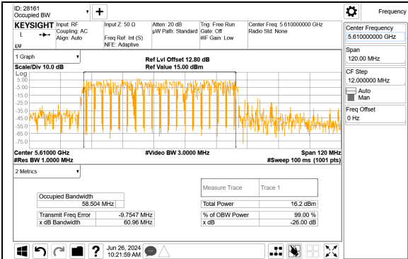
80MHz – 484+242T – Mid Channel – Puncture Pattern 8 – (UNII-2c) – Ant 6
