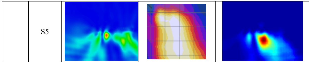
Figure 7. Simulated and measured point PD for different beams for n258.
