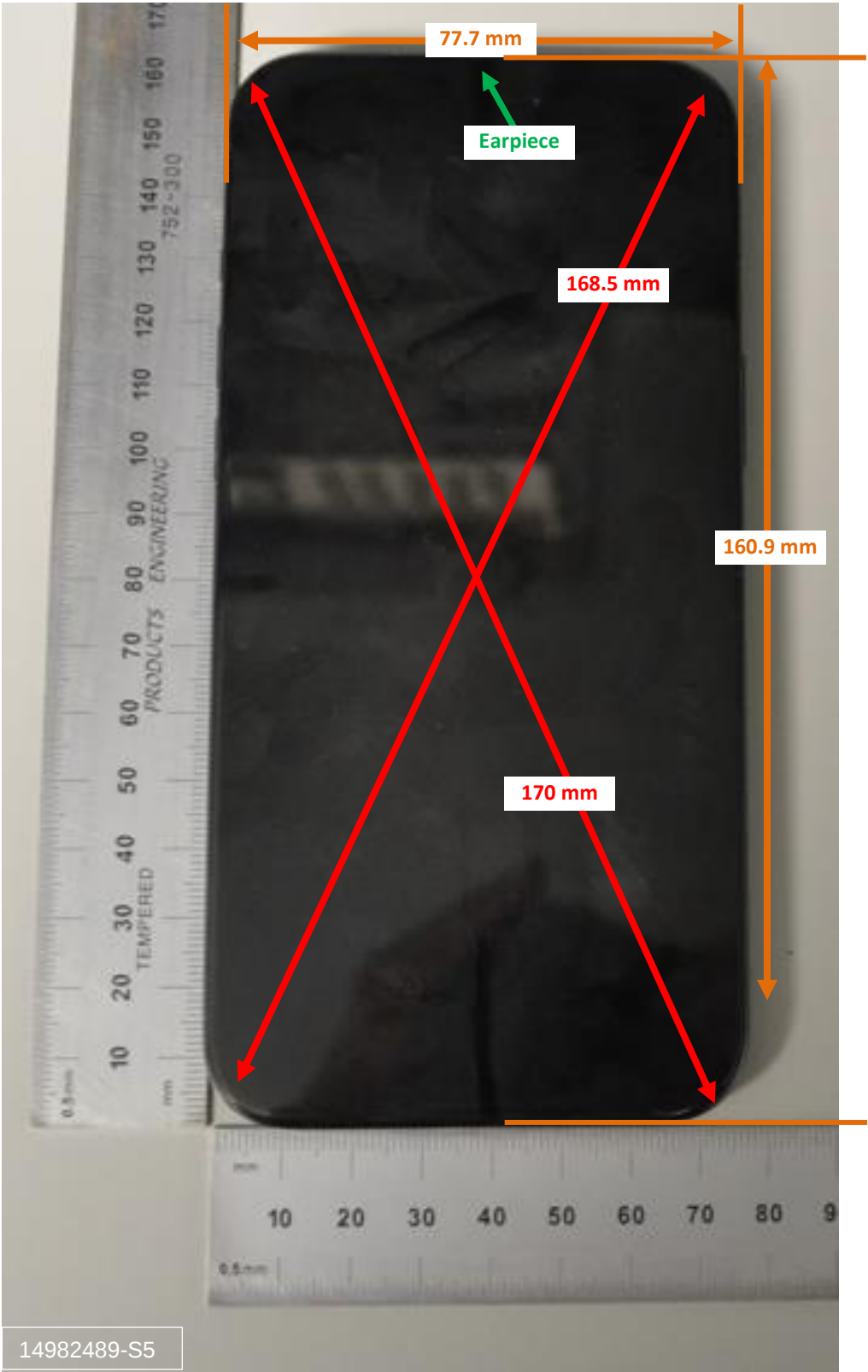
Photograph 1: Overall Dimensions
