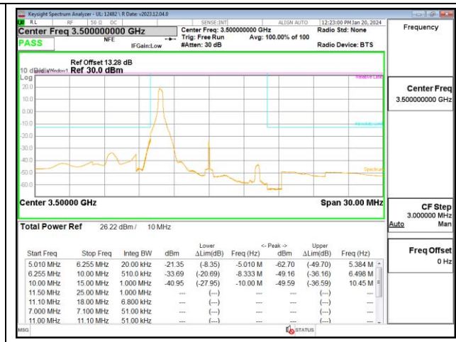
5G NR n77 10MHz BPSK Middle Channel RB1-0
