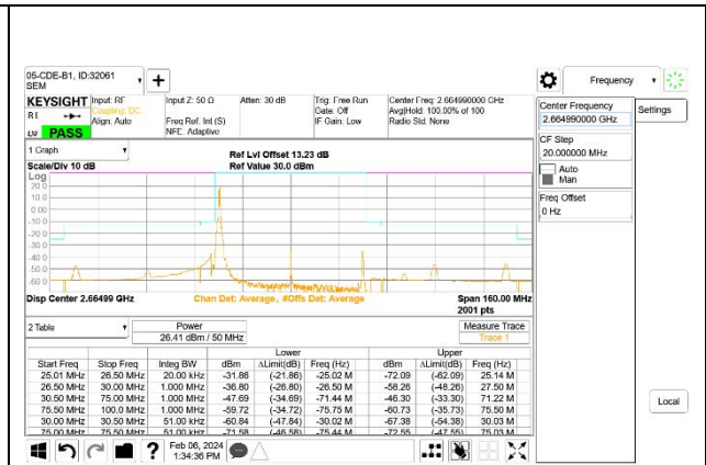
5G NR n41 50MHz BPSK High Channel RB1-0
