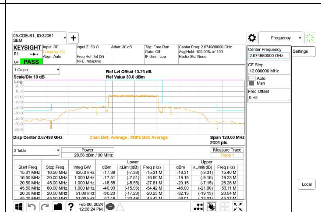
5G NR n41 30MHz BPSK High Channel RB75-0
