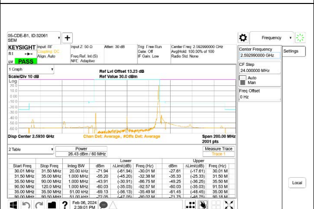
5G NR n41 60MHz BPSK Middle Channel RB1-161
