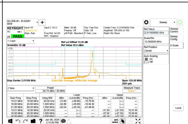
5G NR n41 30MHz BPSK Low Channel RB1-77
