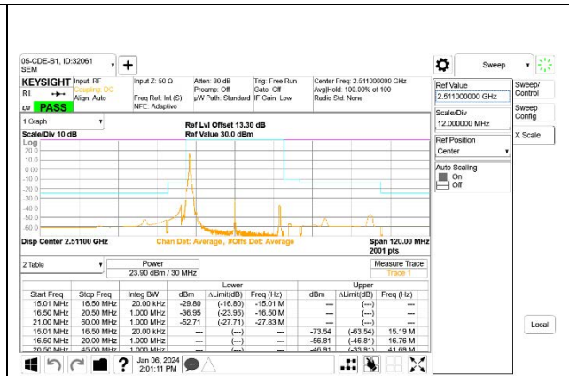
5G NR n41 30MHz BPSK Low Channel RB1-0
