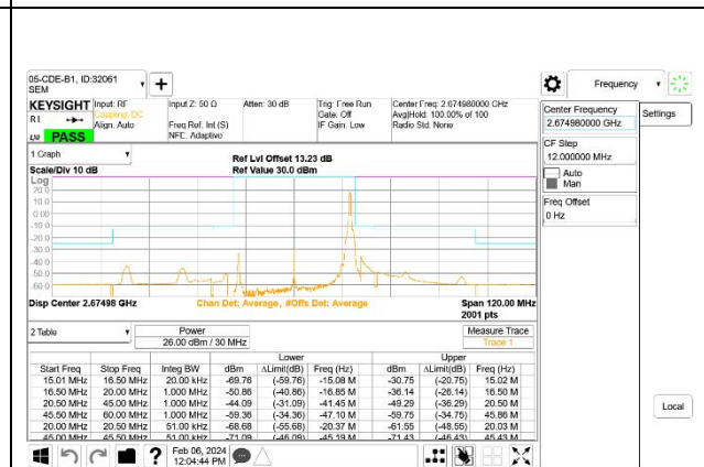
5G NR n41 30MHz BPSK High Channel RB1-77
