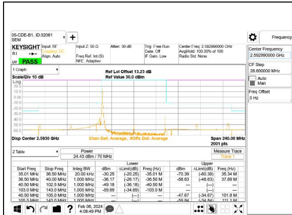
5G NR n41 70MHz BPSK Middle Channel RB1-0
