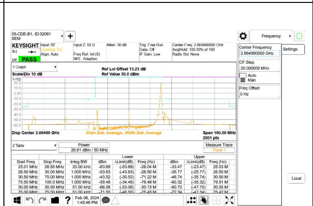
5G NR n41 50MHz BPSK High Channel RB1-132
