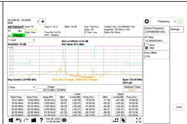
5G NR n41 30MHz BPSK High Channel RB1-0
