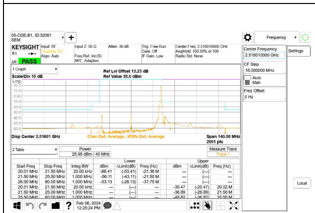
5G NR n41 40MHz BPSK Low Channel RB1-105
