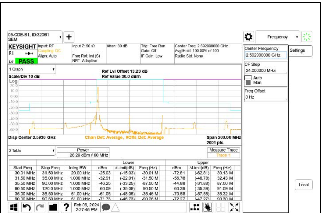
5G NR n41 60MHz BPSK Middle Channel RB1-0
