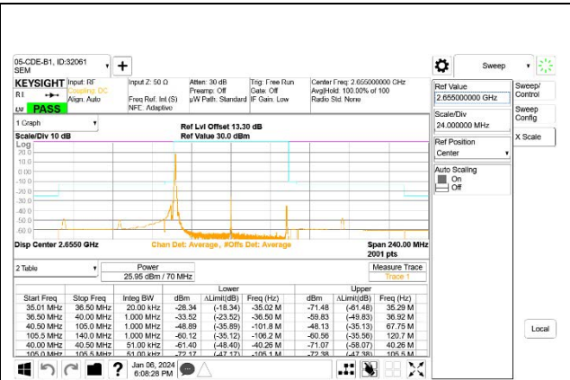
5G NR n41 70MHz BPSK High Channel RB1-0
