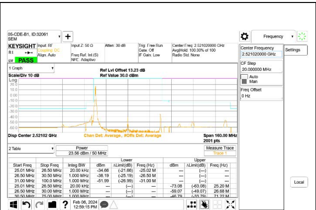
5G NR n41 50MHz BPSK Low Channel RB1-0
