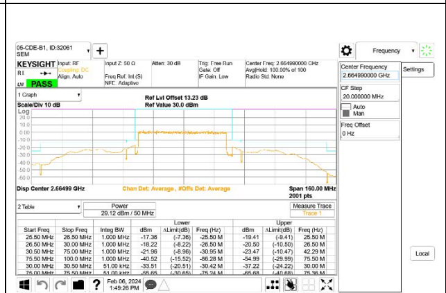
5G NR n41 50MHz BPSK High Channel RB128-0
