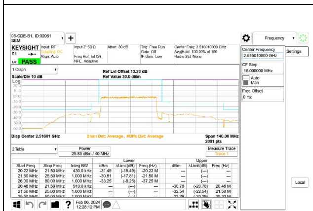
5G NR n41 40MHz BPSK Low Channel RB100-0
