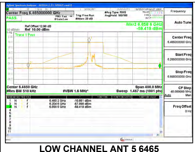
LOW CHANNEL ANT 5 6465
