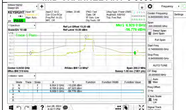
HIGH CHANNEL ANT 6 6845
