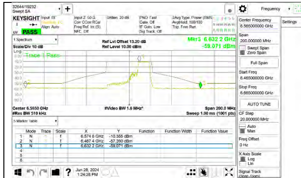
LOW CHANNEL ANT 6 6565
