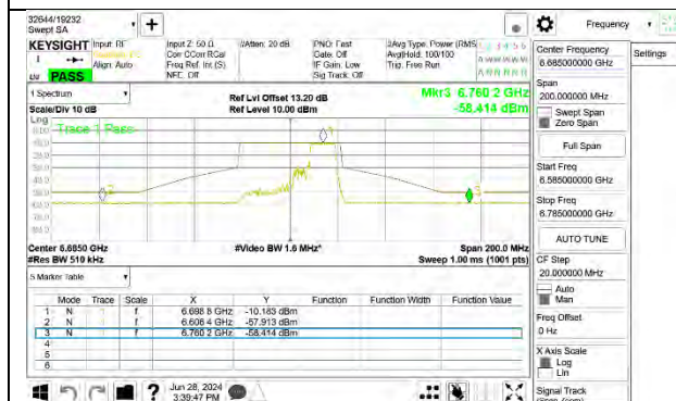
MID CHANNEL ANT 6 6685
