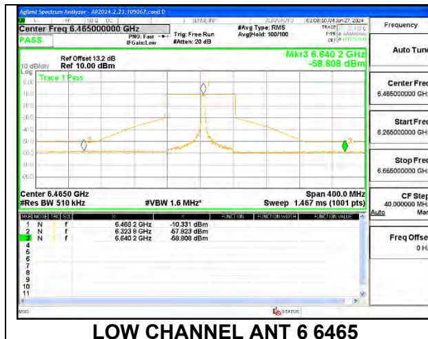
LOW CHANNEL ANT 6 6465
