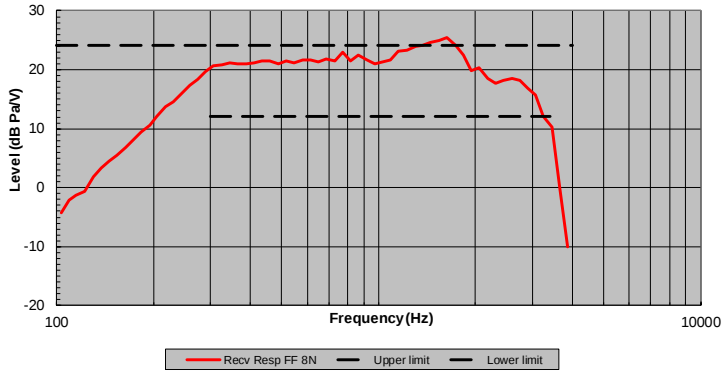
TIA-5050 Free Field Measurement at 8N Receive Frequency Response
