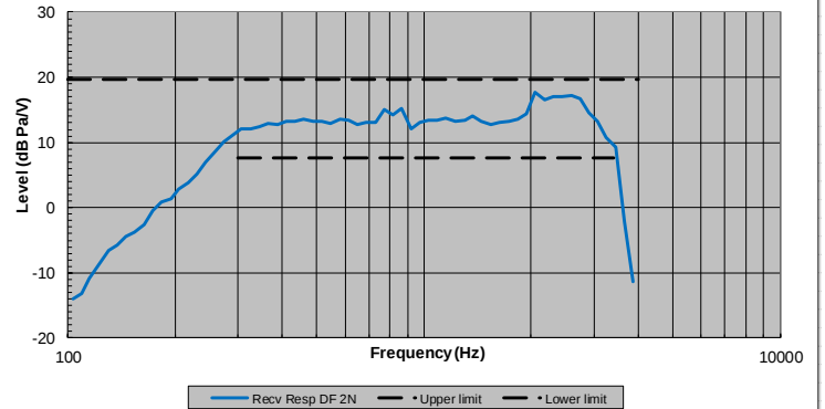
TIA-5050 Diffuse Field Measurement at 2N Receive Frequency Response
