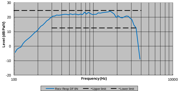
TIA-5050 Diffuse Field Measurement at 8N Receive Frequency Response
