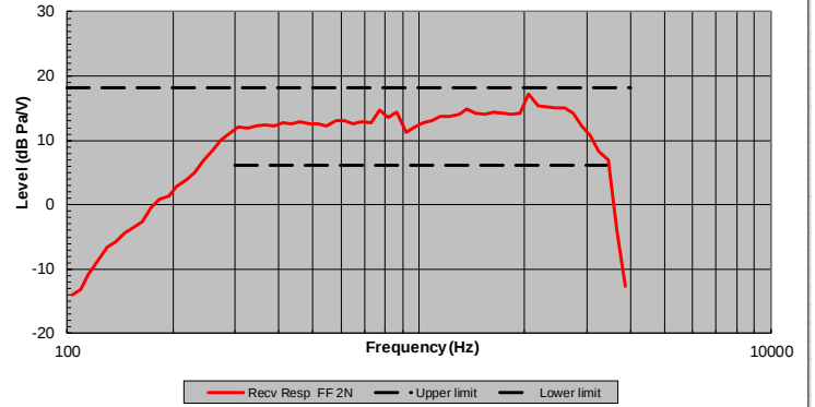
TIA-5050 Free Field Measurement at 2N Receive Frequency Response
