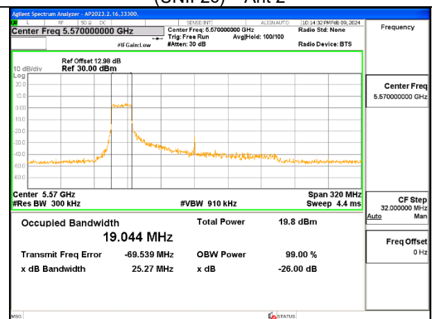
160MHz - Mid Channel – 242T-RU61 (UNII-2c) – Ant 2
