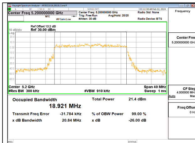
20MHz - Mid Channel - SU (UNII-1) - Ant 1
