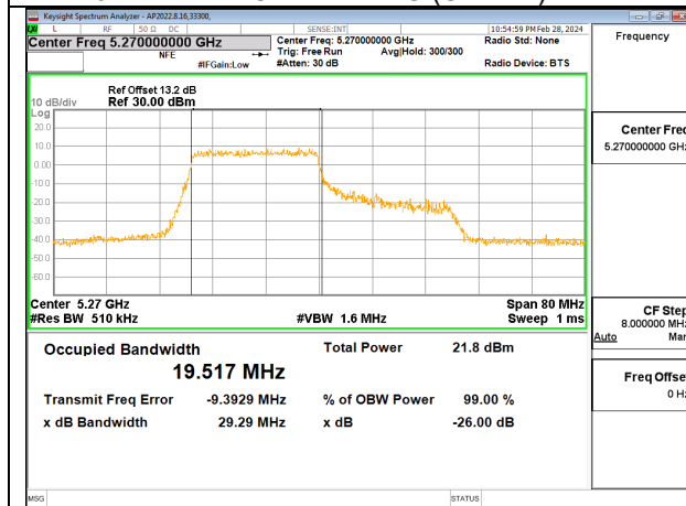
40MHz - Low Channel - 242T-RU61(UNII-2a) - Ant 1
