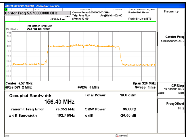
160MHz - Mid Channel – SU (UNII-2c) – Ant 2
