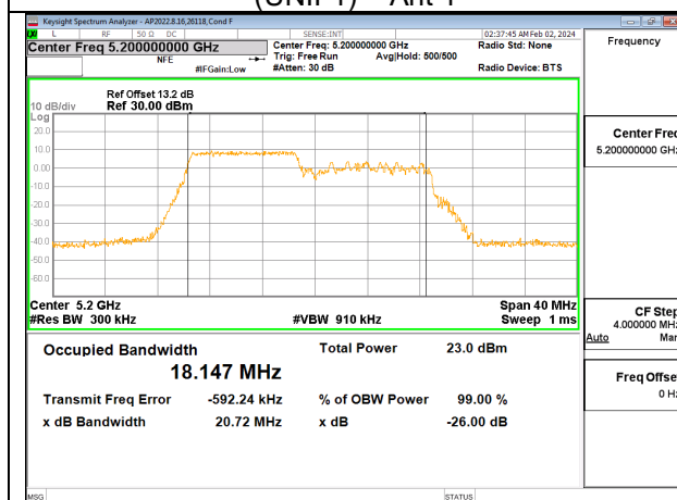
20MHz - Mid Channel - 106T-RU53 (UNII-1) - Ant 1
