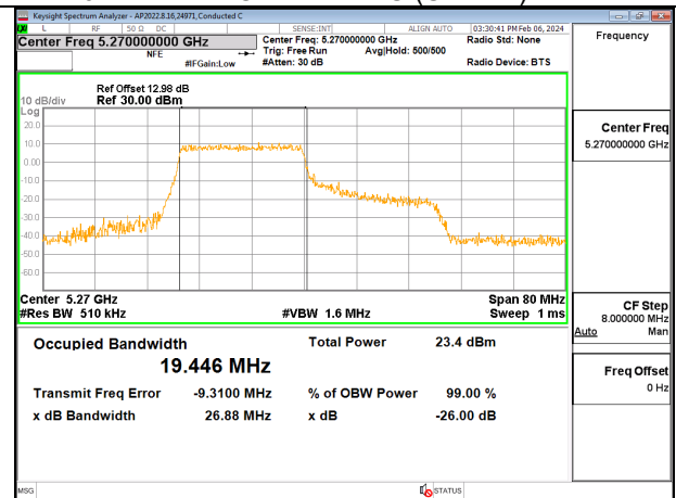
40MHz - Low Channel - 242T-RU61(UNII-2a) - Ant 2
