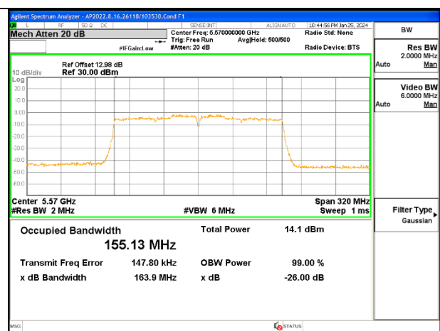
160MHz - Mid Channel (UNII-2c) - Ant 2
