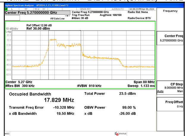
40MHz - Low Channel - 52T-RU37 (UNII-2a) - Ant 2
