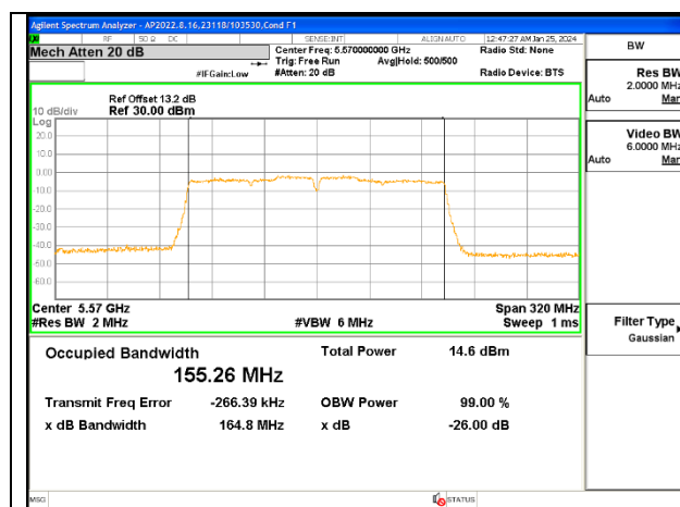
160MHz - Mid Channel (UNII-2c) - Ant 1
