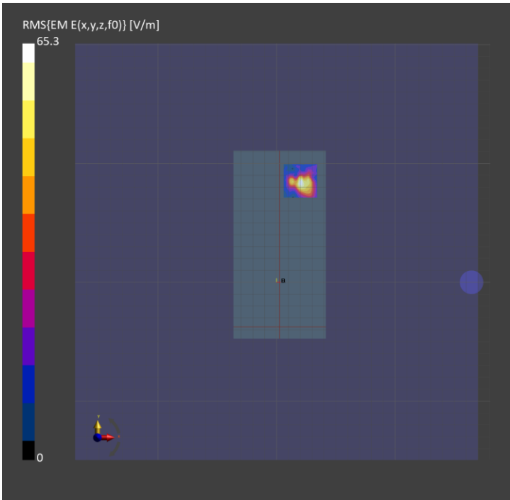
Figure 6-2: Band n260, Beam ID 141, point PD and 4cm² PD, Right
