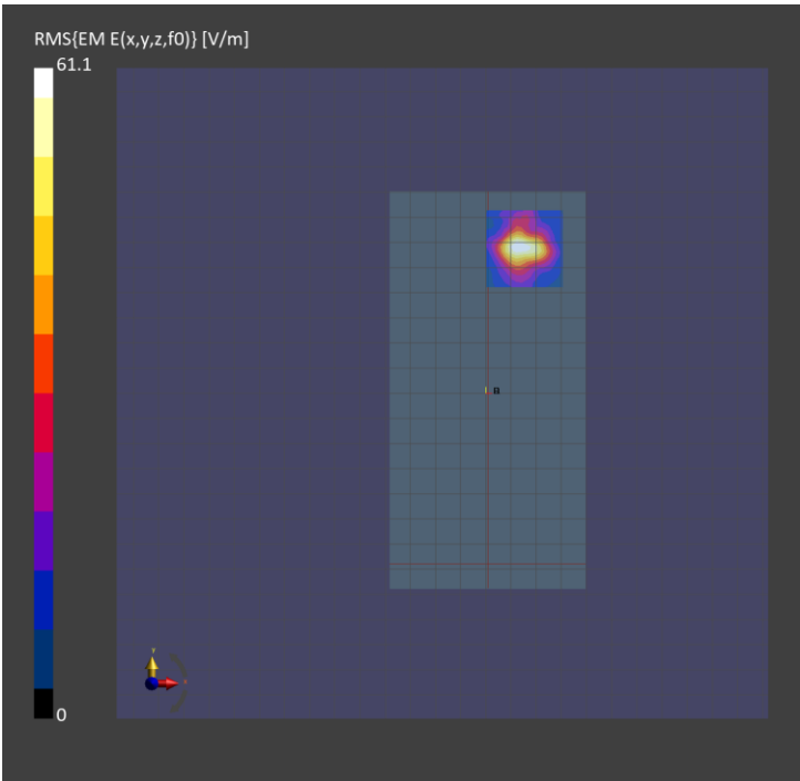
Figure 6-1: Band n258, Beam ID 14, point PD and 4cm² PD, Back
