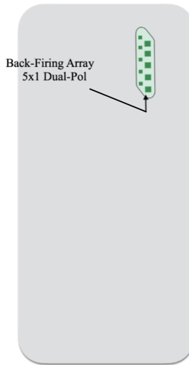
Figure 4. Schematic of the simulation model consisting of a back-firing 5G antenna array.
