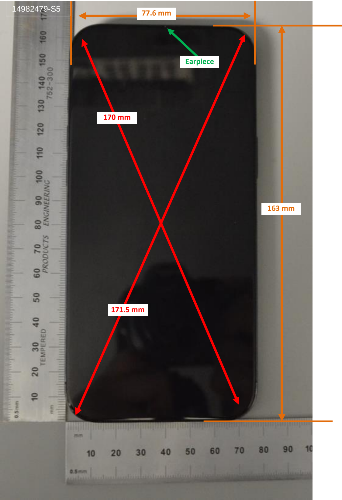
Photograph 1: Overall Dimensions
