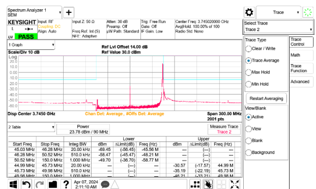
5G NR n77 90MHz BPSK Low Channel RB1-244 Port B ID 27342
