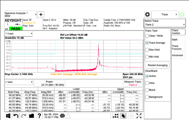
5G NR n77 80MHz BPSK Low Channel RB1-216 Port B ID 27342
