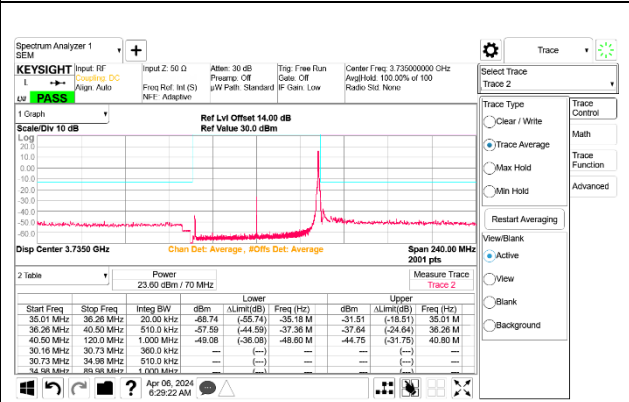
5G NR n77 70MHz BPSK Low Channel RB1-188 Port B ID 27342
