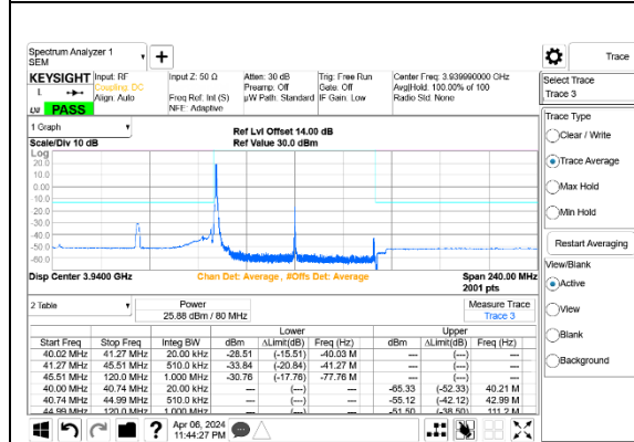
5G NR n77 80MHz BPSK High Channel RB1-0 Port A+B ID 27342
