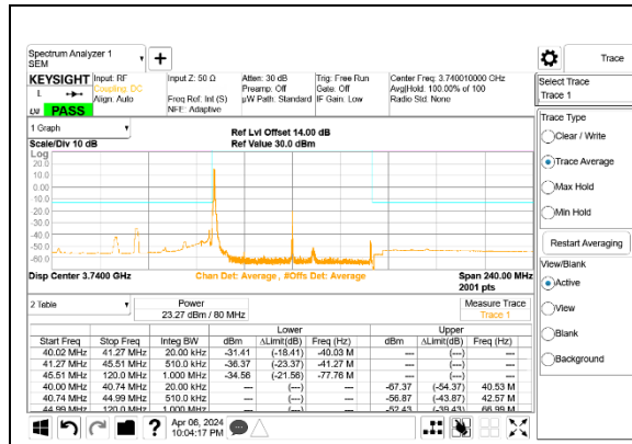
5G NR n77 80MHz BPSK Low Channel RB1-0 Port A ID 27342
