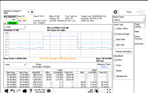
5G NR n77 60MHz BPSK Mid Channel RB162-0 Port A+B
