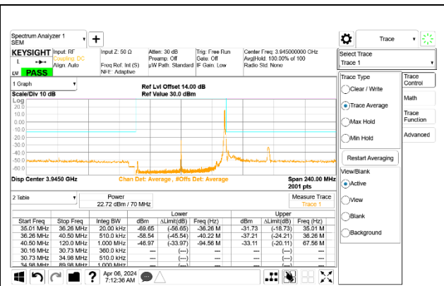
5G NR n77 70MHz BPSK High Channel RB1-188 Port A ID 27342
