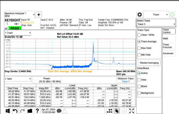
5G NR n77 80MHz BPSK High Channel RB1-216 Port A+B ID 27342
