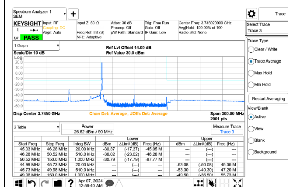
5G NR n77 90MHz BPSK Low Channel RB1-0 Port A+B ID 27342
