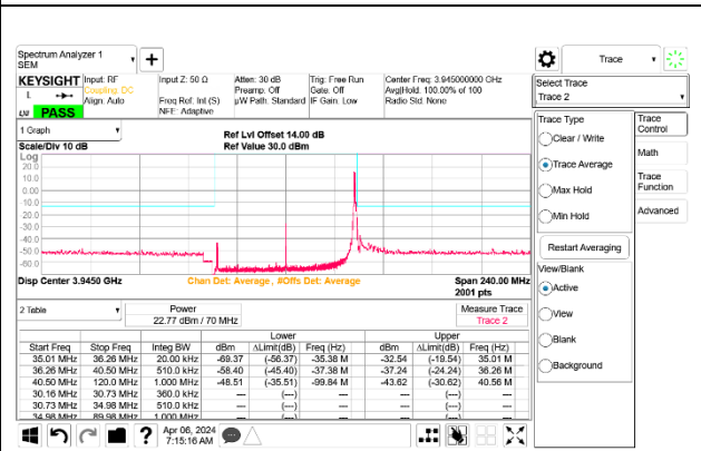
5G NR n77 70MHz BPSK High Channel RB1-188 Port B ID 27342
