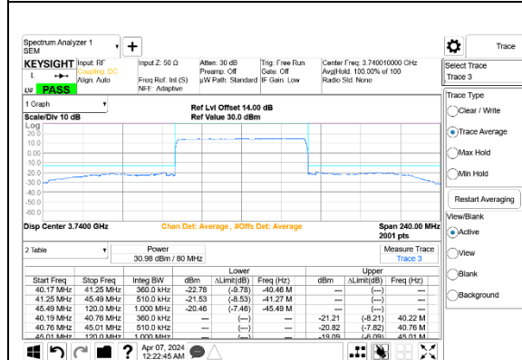
5G NR n77 80MHz BPSK Low Channel RB216-0 Port A+B ID 27342
