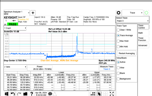
5G NR n77 70MHz BPSK Low Channel RB1-188 Port A+B ID 27342
