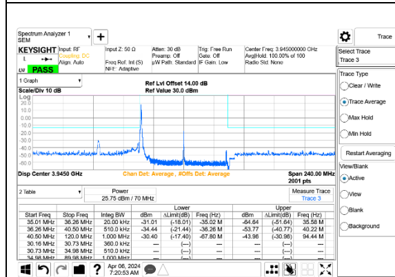
5G NR n77 70MHz BPSK High Channel RB1-0 Port A+B ID 27342
