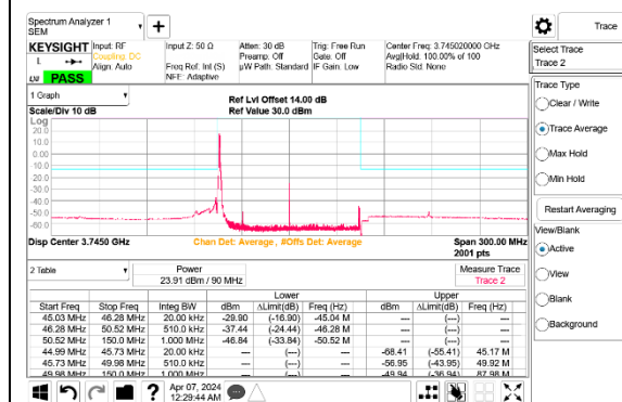
5G NR n77 90MHz BPSK Low Channel RB1-0 Port B ID 27342
