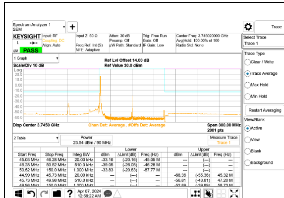
5G NR n77 90MHz BPSK Low Channel RB1-0 Port A ID 27342
