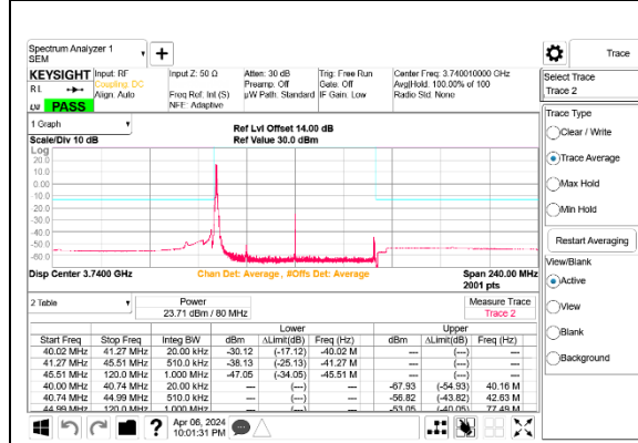
5G NR n77 80MHz BPSK Low Channel RB1-0 Port B ID 27342
