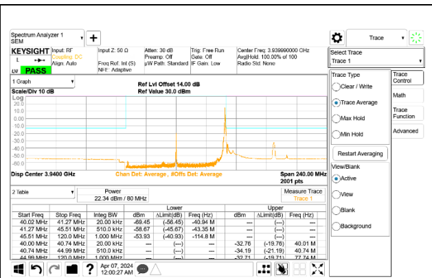
5G NR n77 80MHz BPSK High Channel RB1-216 Port A ID 27342
