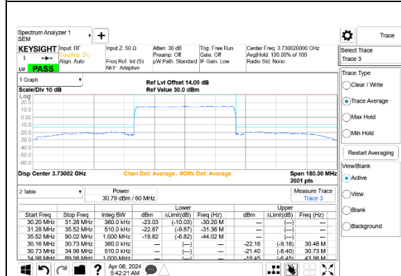
5G NR n77 60MHz BPSK Low Channel RB162-0 Port A+B
