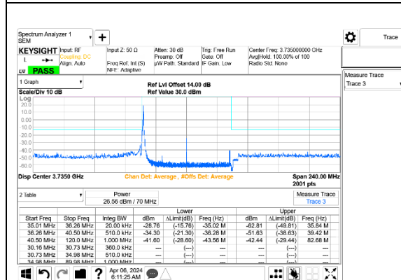
5G NR n77 70MHz BPSK Low Channel RB1-0 Port A+B ID 27342
