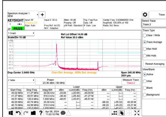
5G NR n77 80MHz BPSK High Channel RB1-0 Port B ID 27342
