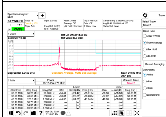
5G NR n77 70MHz BPSK High Channel RB1-0 Port B ID 27342
