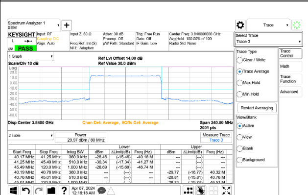
5G NR n77 80MHz BPSK Mid Channel RB216-0 Port A+B ID 27342
