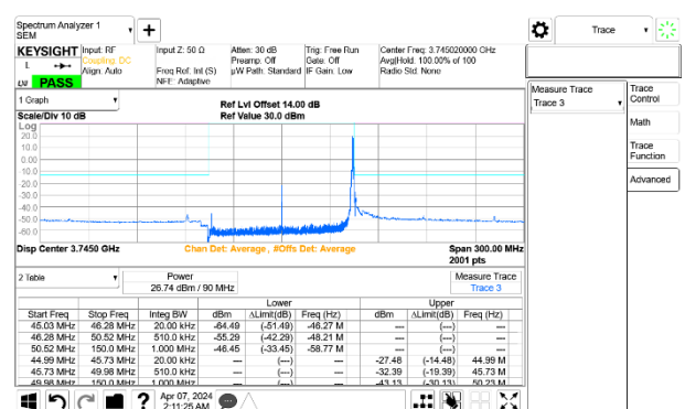
5G NR n77 90MHz BPSK Low Channel RB1-244 Port A+B ID 27342
