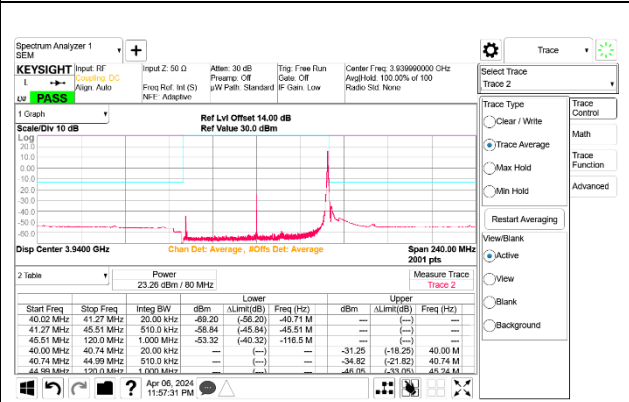
5G NR n77 80MHz BPSK High Channel RB1-216 Port B ID 27342
