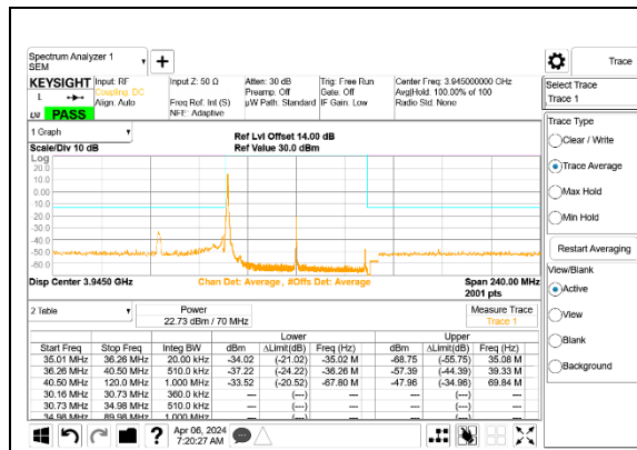
5G NR n77 70MHz BPSK High Channel RB1-0 Port A ID 27342
