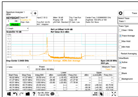
5G NR n77 80MHz BPSK High Channel RB1-0 Port A ID 27342
