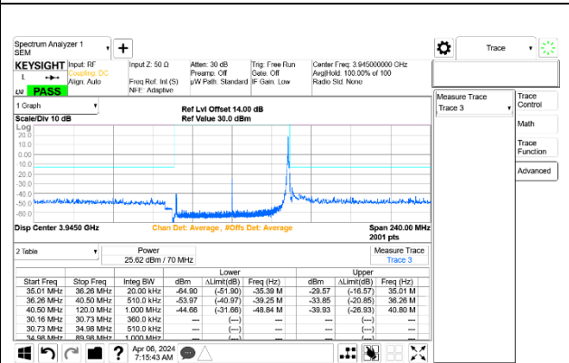
5G NR n77 70MHz BPSK High Channel RB1-188 Port A+B ID 27342
