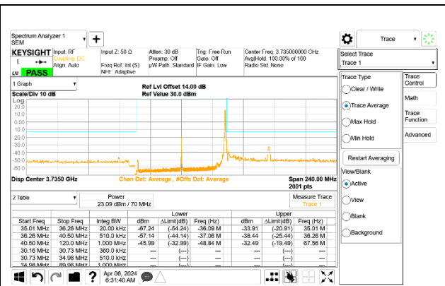
5G NR n77 70MHz BPSK Low Channel RB1-188 Port A ID 27342
