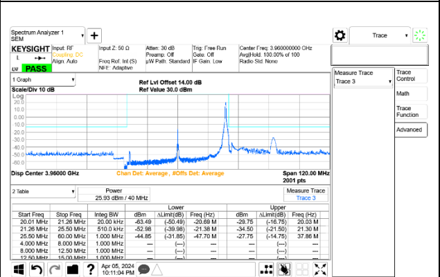
5G NR n77 40MHz BPSK High Channel RB1-105 Port A+B ID 27342
