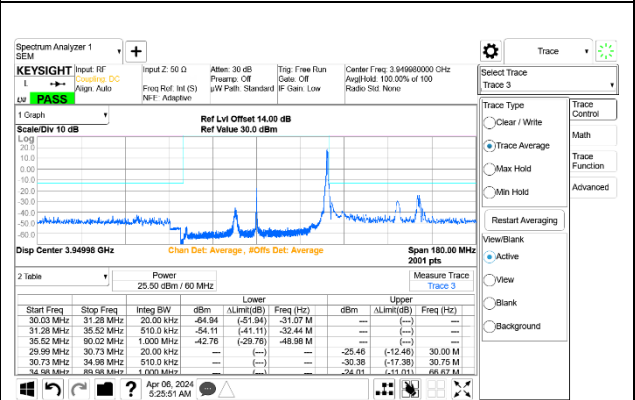
5G NR n77 60MHz BPSK High Channel RB1-161 Port A+B ID 27342
