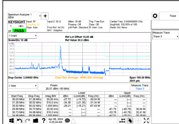
5G NR n77 60MHz BPSK Middle Channel RB1-0 Port A+B
