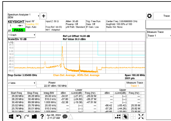
5G NR n77 50MHz BPSK High Channel RB1-0 Port A ID 27342
