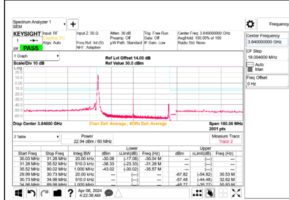
5G NR n77 60MHz BPSK Middle Channel RB1-0 Port B
