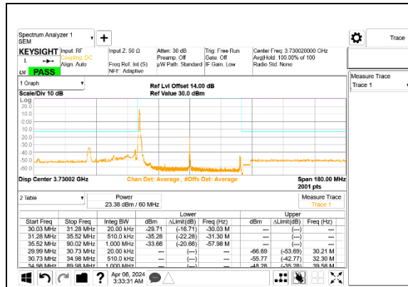
5G NR n77 60MHz BPSK Low Channel RB1-0 Port A ID 27342
