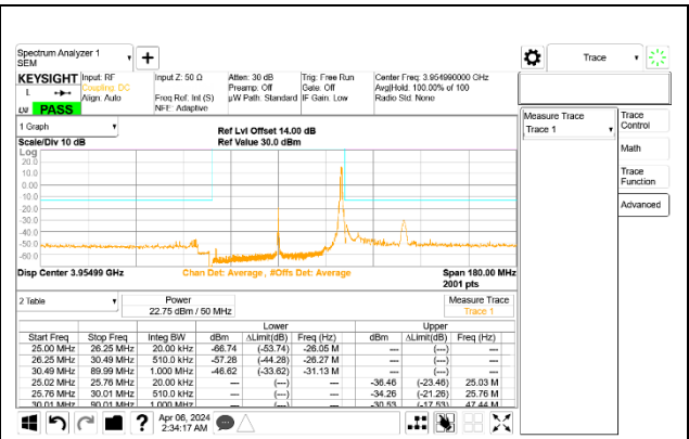
5G NR n77 50MHz BPSK High Channel RB1-132 Port A ID 27342
