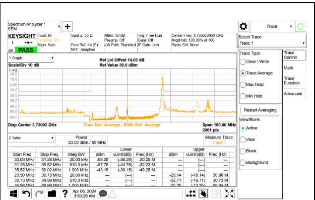
5G NR n77 60MHz BPSK Low Channel RB1-161 Port A ID 27342
