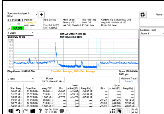
5G NR n77 60MHz BPSK High Channel RB1-0 Port A+B ID 27342
