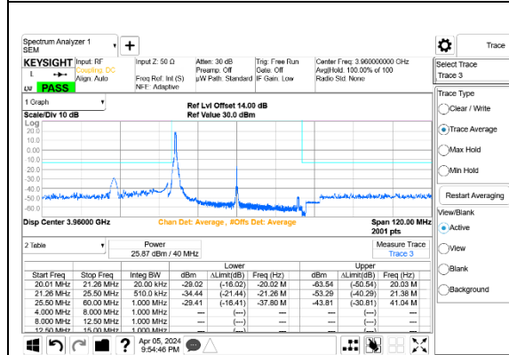
5G NR n77 40MHz BPSK High Channel RB1-0 Port A+B ID 27342
