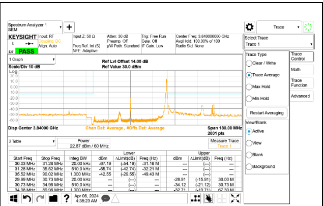
5G NR n77 60MHz BPSK Mid Channel RB1-161 Port A
