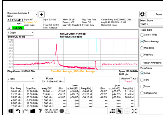
5G NR n77 40MHz BPSK High Channel RB1-0 Port B ID 27342
