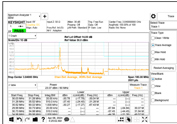
5G NR n77 60MHz BPSK Middle Channel RB1-0 Port A
