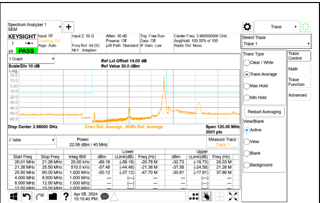
5G NR n77 40MHz BPSK High Channel RB1-105 Port A ID 27342
