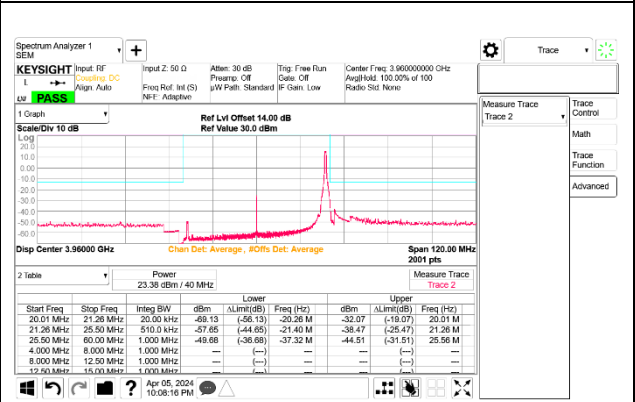
5G NR n77 40MHz BPSK High Channel RB1-105 Port B ID 27342
