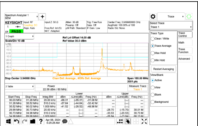
5G NR n77 60MHz BPSK High Channel RB1-161 Port A ID 27342
