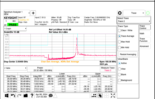
5G NR n77 50MHz BPSK High Channel RB1-132 Port B ID 27342
