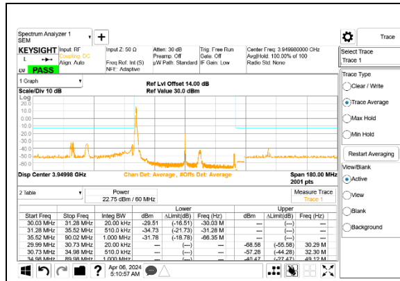
5G NR n77 60MHz BPSK High Channel RB1-0 Port A ID 27342
