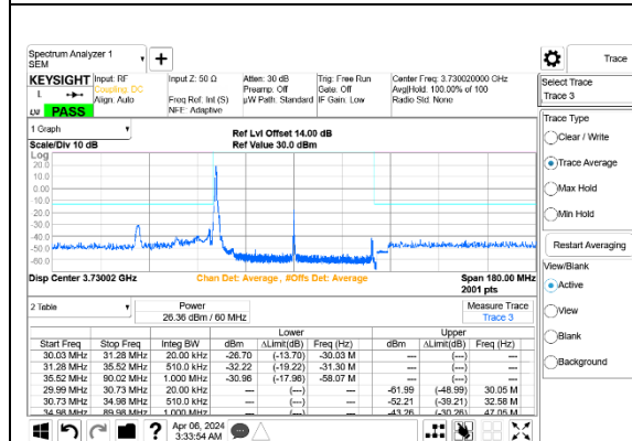
5G NR n77 60MHz BPSK Low Channel RB1-0 Port A+B ID 27342
