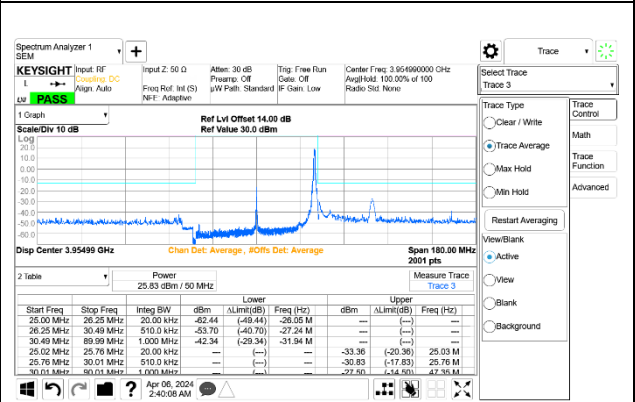
5G NR n77 50MHz BPSK High Channel RB1-132 Port A+B ID 27342
