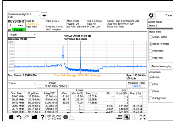
5G NR n77 50MHz BPSK High Channel RB1-0 Port A+B ID 27342
