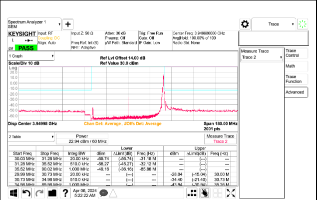
5G NR n77 60MHz BPSK High Channel RB1-161 Port B ID 27342
