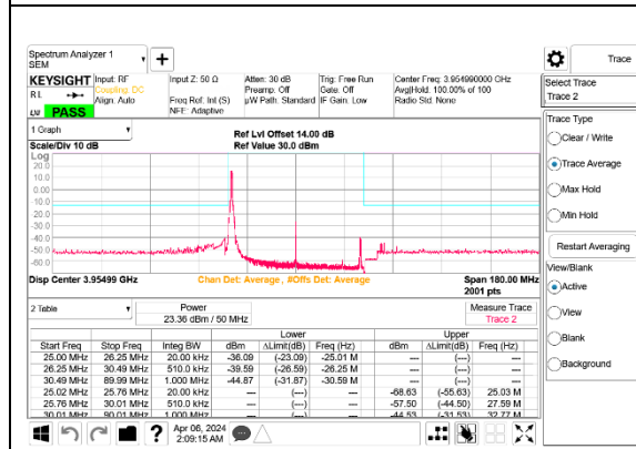
5G NR n77 50MHz BPSK High Channel RB1-0 Port B ID 27342
