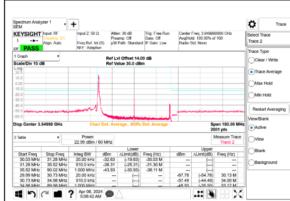
5G NR n77 60MHz BPSK High Channel RB1-0 Port B ID 27342
