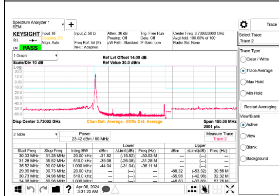
5G NR n77 60MHz BPSK Low Channel RB1-0 Port B ID 27342
