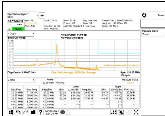
5G NR n77 40MHz BPSK High Channel RB1-0 Port A ID 27342
