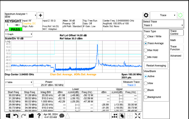
5G NR n77 60MHz BPSK Mid Channel RB1-161 Port A+B
