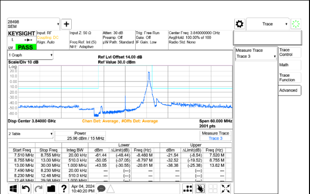
5G NR n77 15MHz BPSK Mid Channel RB1-37 Port A+B ID 28498
