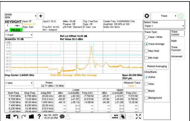
5G NR n77 15MHz BPSK Mid Channel RB1-37 Port A ID 28498
