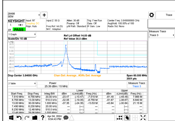
5G NR n77 15MHz BPSK Middle Channel RB1-0 Port A+B ID 28498
