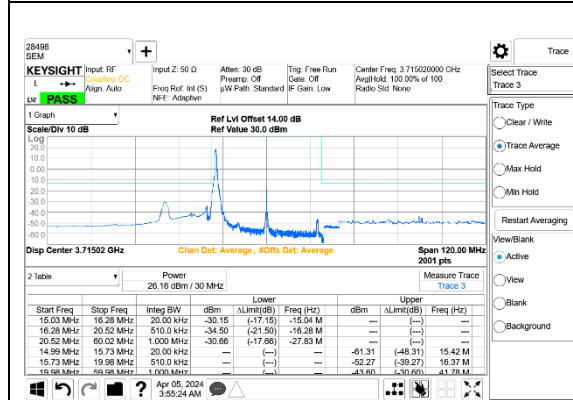
5G NR n77 30MHz BPSK Low Channel RB1-0 Port A+B
