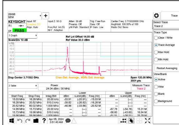
5G NR n77 30MHz BPSK Low Channel RB1-0 Port B
