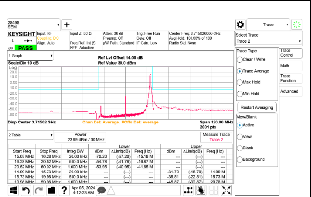
5G NR n77 30MHz BPSK Low Channel RB1-77 Port B
