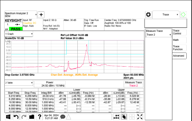
5G NR n77 10MHz BPSK High Channel RB1-23 Port B ID 27342
