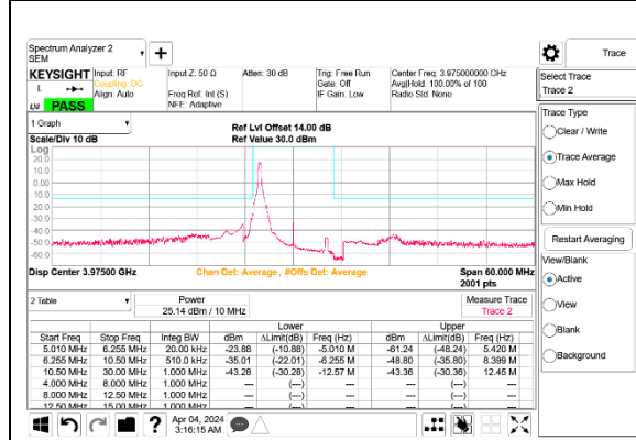
5G NR n77 10MHz BPSK High Channel RB1-0 Port B ID 27342
