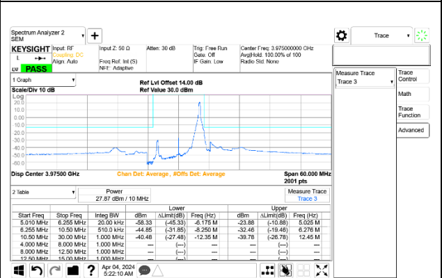
5G NR n77 10MHz BPSK High Channel RB1-23 Port A+B ID 27342
