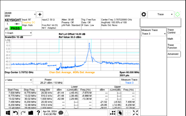
5G NR n77 15MHz BPSK Low Channel RB1-37 Port A+B ID 28498
