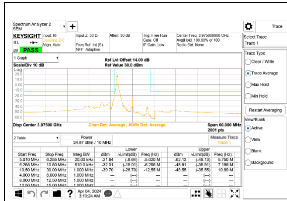
5G NR n77 10MHz BPSK High Channel RB1-0 Port A ID 27342
