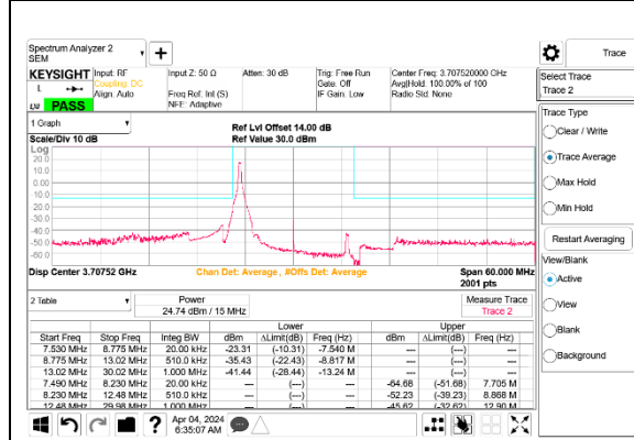
5G NR n77 15MHz BPSK Low Channel RB1-0 Port B ID 27342
