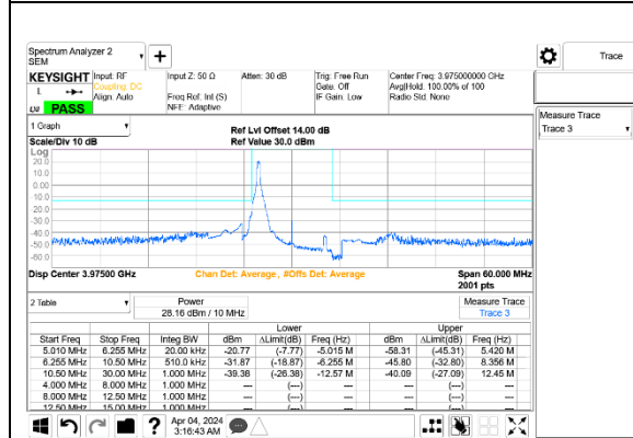
5G NR n77 10MHz BPSK High Channel RB1-0 Port A+B ID 27342
