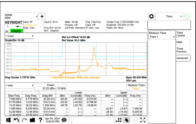
5G NR n77 15MHz BPSK Low Channel RB1-37 Port A ID 28498
