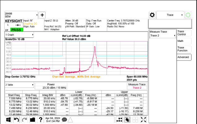
5G NR n77 15MHz BPSK Low Channel RB1-37 Port B ID 28498
