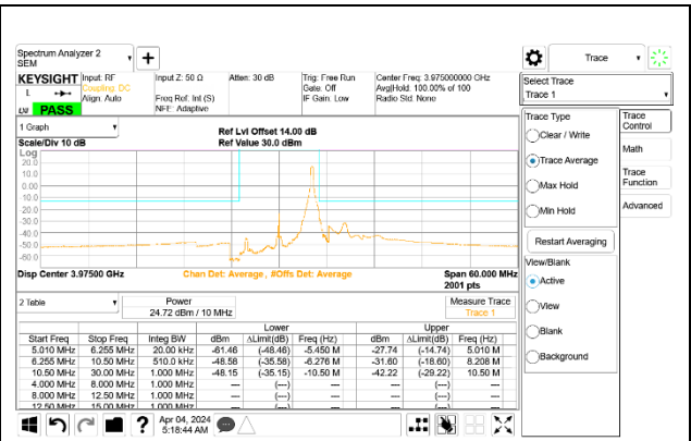
5G NR n77 10MHz BPSK High Channel RB1-23 Port A ID 27342
