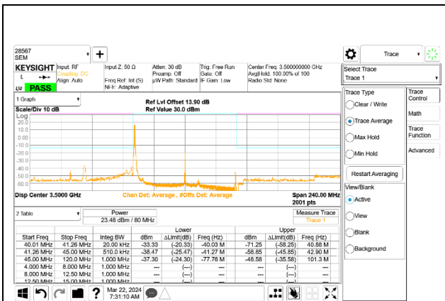
5G NR n77 80MHz BPSK Middle Channel RB1-0 Port A
