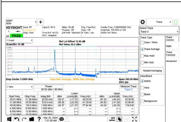
5G NR n77 80MHz BPSK Middle Channel RB1-0 Port A+B
