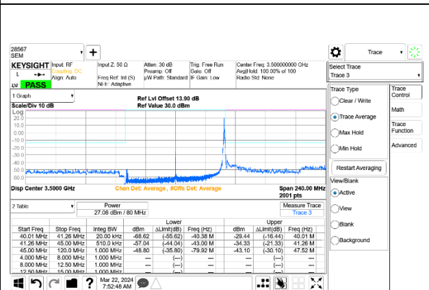
5G NR n77 80MHz BPSK Mid Channel RB1-216 Port A+B
