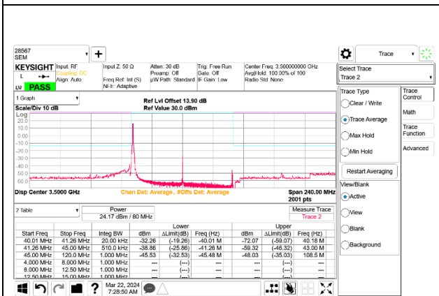
5G NR n77 80MHz BPSK Middle Channel RB1-0 Port B
