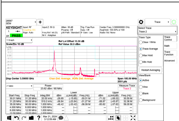
5G NR n77 60MHz BPSK Middle Channel RB1-0 Port B
