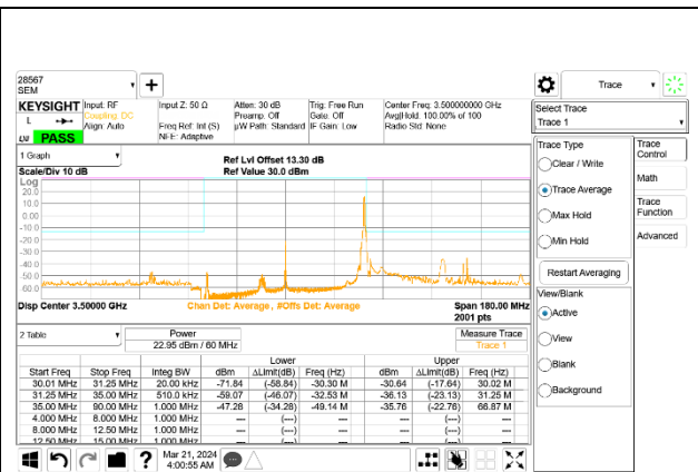
5G NR n77 60MHz BPSK Mid Channel RB1-161 Port A
