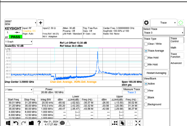
5G NR n77 60MHz BPSK Mid Channel RB1-161 Port A+B
