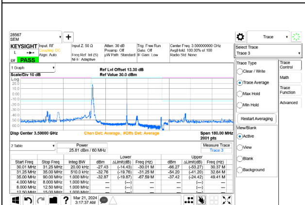
5G NR n77 60MHz BPSK Middle Channel RB1-0 Port A+B
