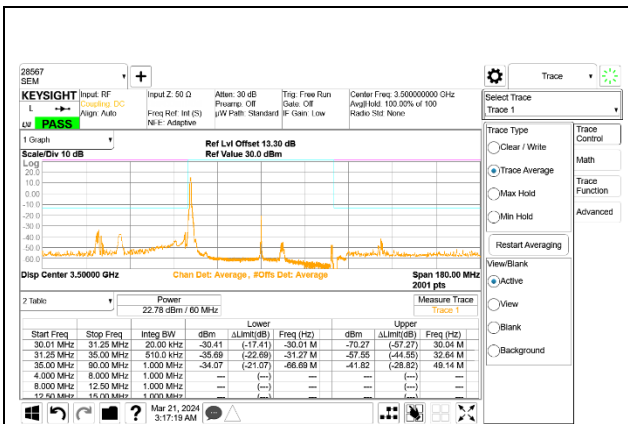
5G NR n77 60MHz BPSK Middle Channel RB1-0 Port A
