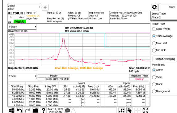
5G NR n77 10MHz BPSK Low Channel RB1-0 Port B
