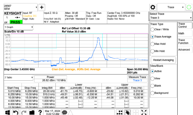
5G NR n77 10MHz BPSK Low Channel RB1-23 Port A+B
