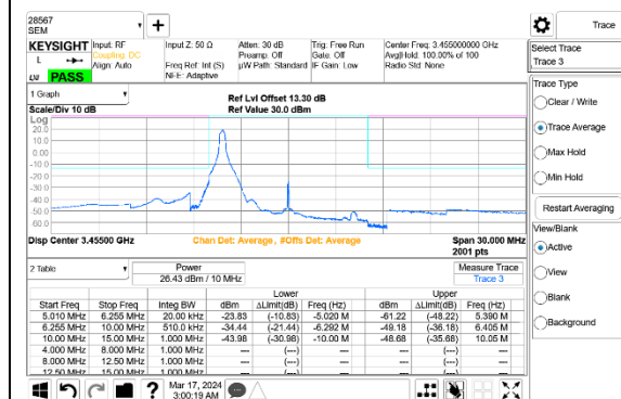
5G NR n77 10MHz BPSK Low Channel RB1-0 Port A+B
