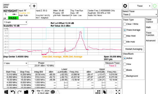
5G NR n77 10MHz BPSK Low Channel RB1-23 Port B
