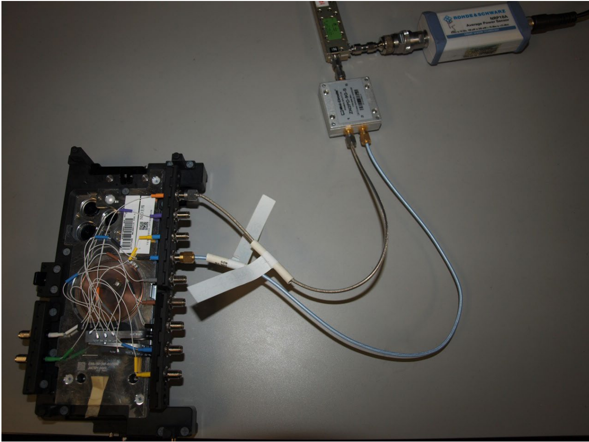
Figure C-2 CMW Conducted power test measurement setup dual port to single Port to call processor, Antenna Switch case
