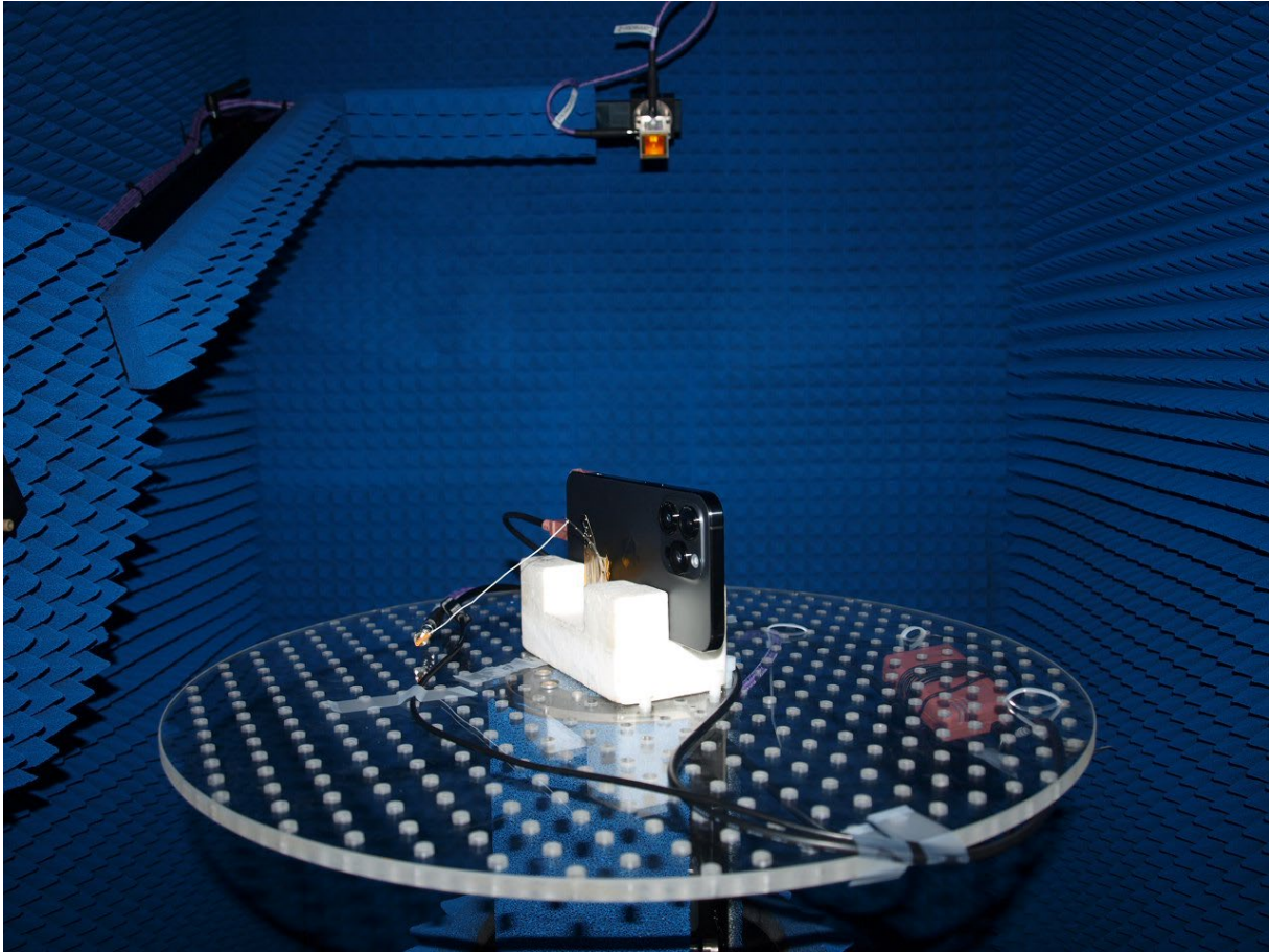
Figure C-6 Conducted Radiated power mmW test measurement setup
