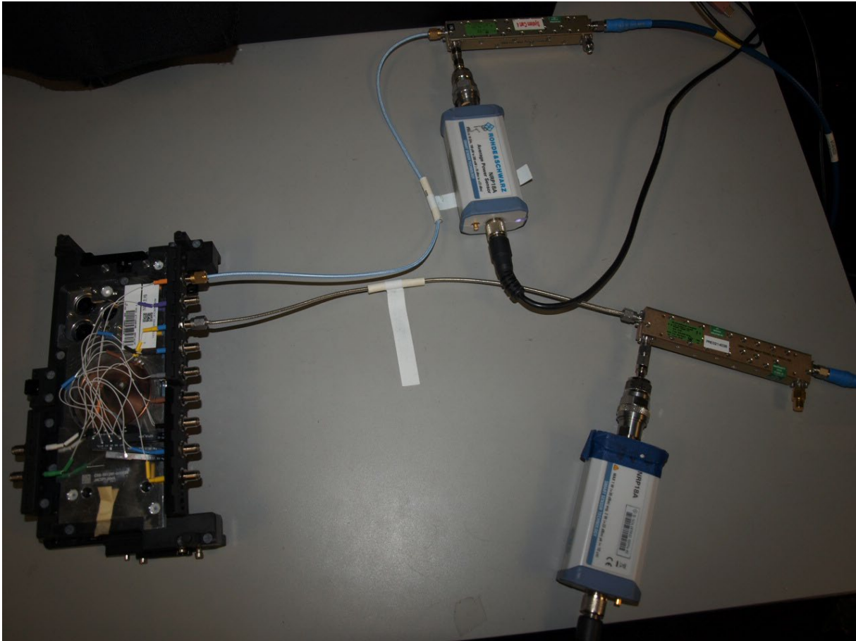
Figure C-4 UXM Conducted power test measurement setup dual port
