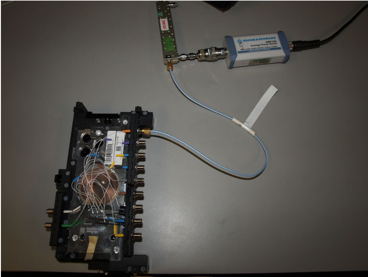
Figure C-1 CMW Conducted power test measurement setup single port
