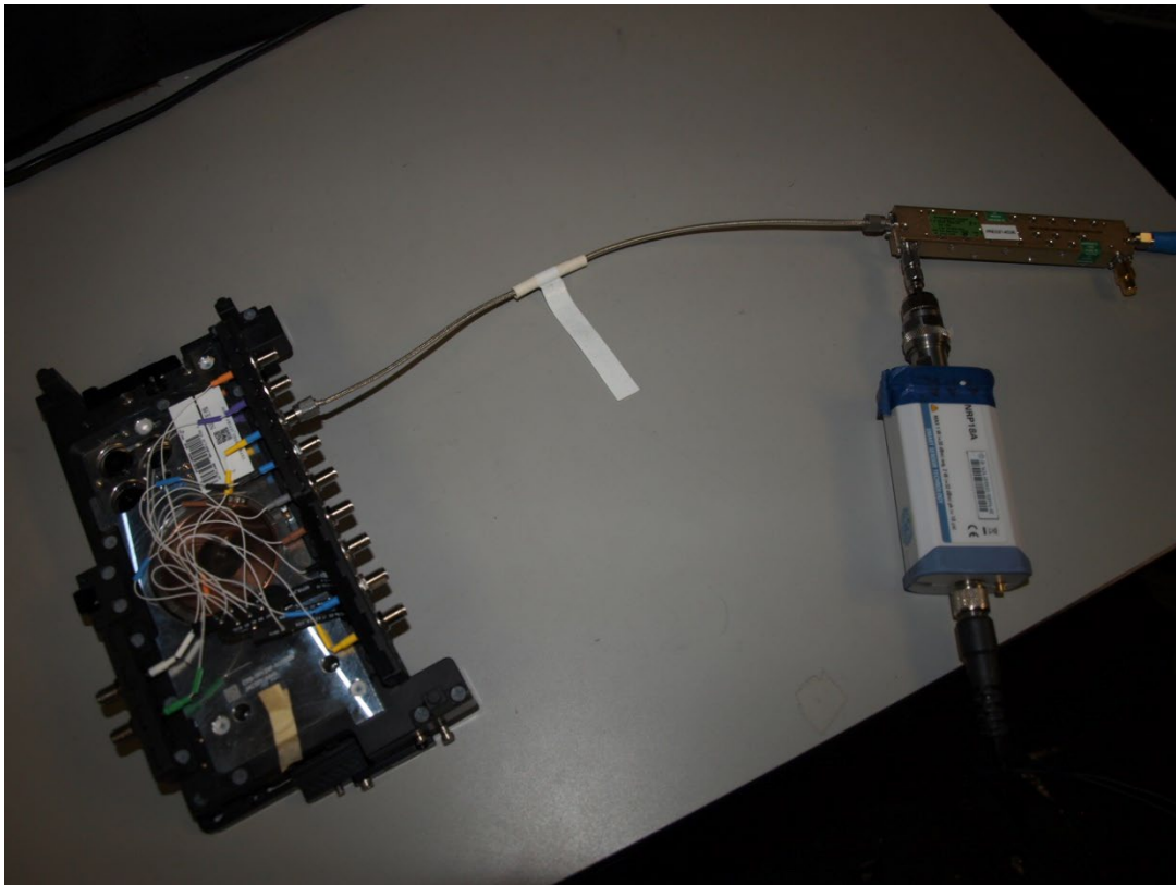
Figure C-3 UXM Conducted power test measurement setup single port
