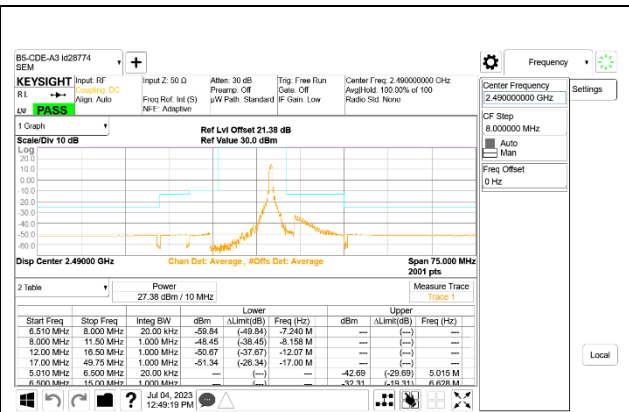
LTE B53 10MHz QPSK High Channel RB1-49
