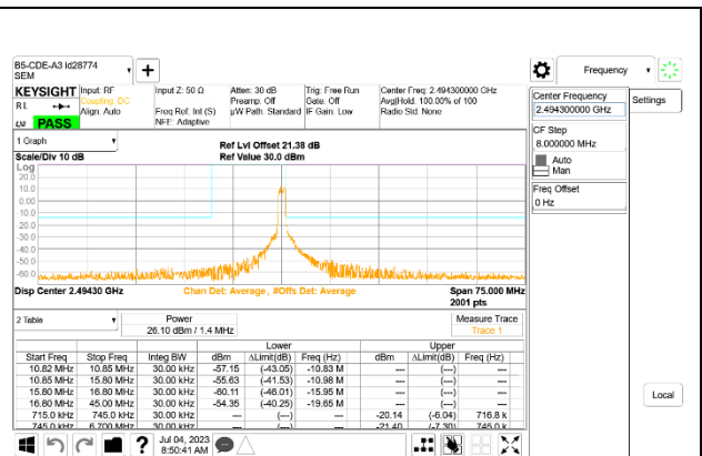
LTE B53 1.4MHz QPSK High Channel RB6-0
