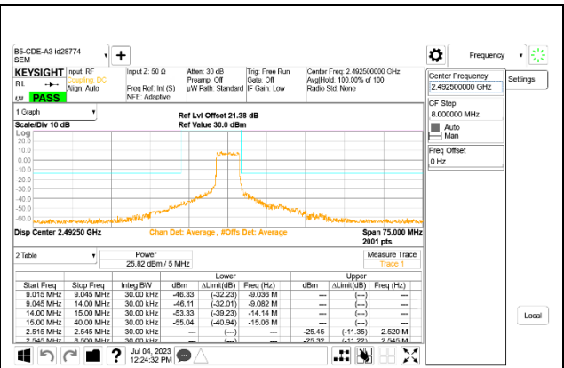
LTE B53 5MHz QPSK High Channel RB25-0
