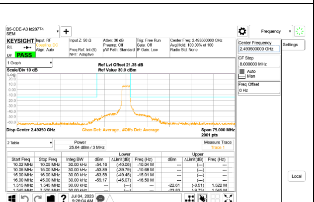
LTE B53 3MHz QPSK High Channel RB15-0
