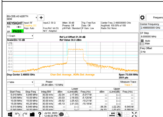
LTE B53 10MHz QPSK Low Channel RB50-0
