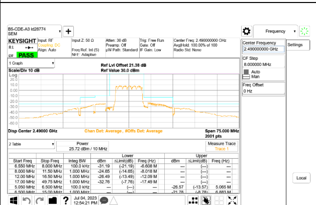
LTE B53 10MHz QPSK High Channel RB50-0
