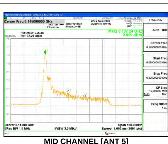
MID CHANNEL [ANT 5]
