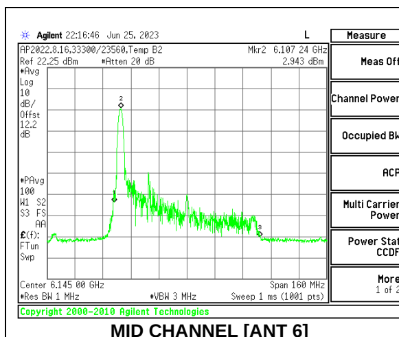
MID CHANNEL [ANT 6]
