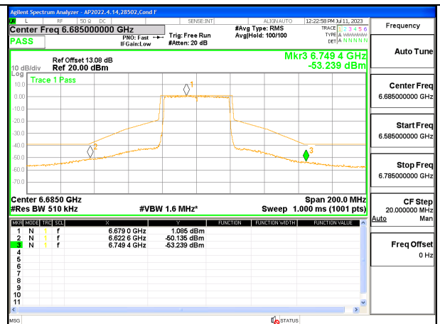
MID CHANNEL 6685
