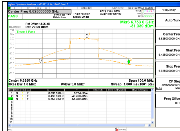
LOW CHANNEL 6625
