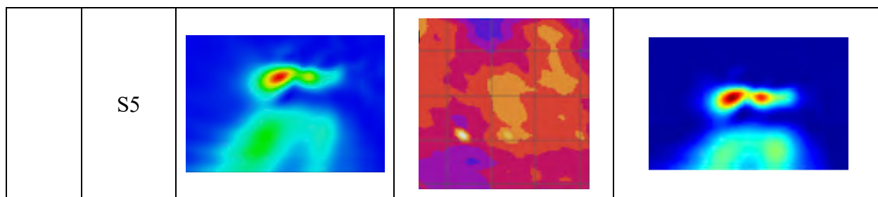
Figure 7. Simulated and measured point PD for different beams for n258
