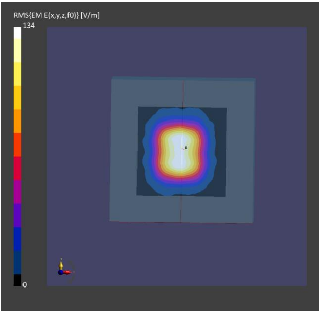
Figure 4-1: 4cm² PD for source validation (worst-case Δ) SAR 3
