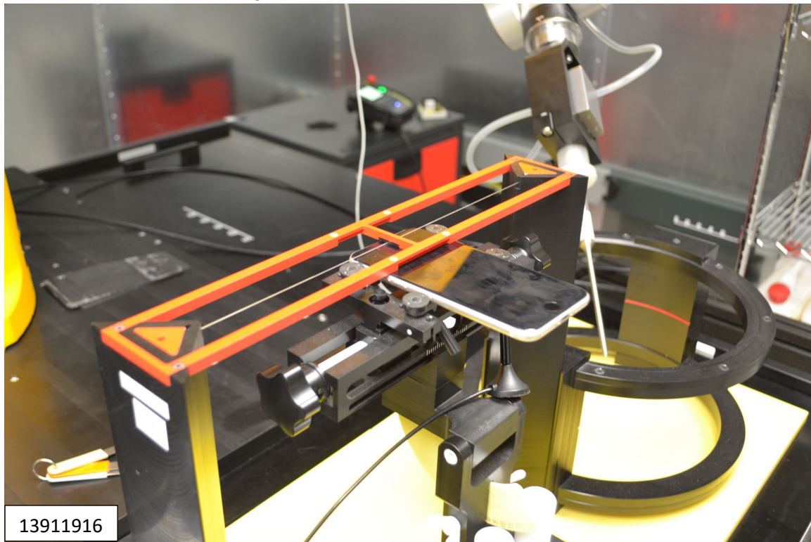
Photograph 1: Front View of the DUT – SAR 9
