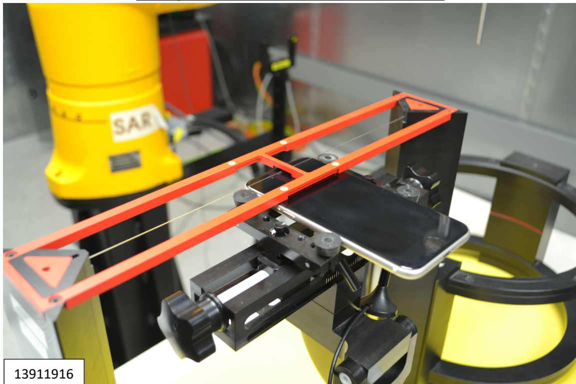
Photograph 2: Front View of the DUT – SAR 11
