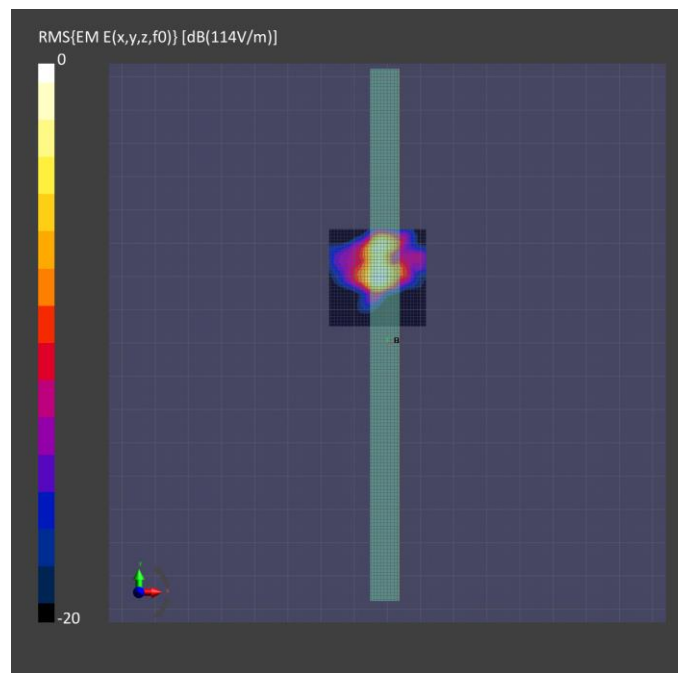
Figure 4-2: Band n260, beam ID 34, 4 cm 2 PD, Edge Right
