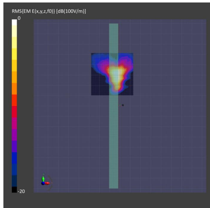
Figure 4-1: Band n258, beam ID 36, 4 cm 2 PD, Edge Right
