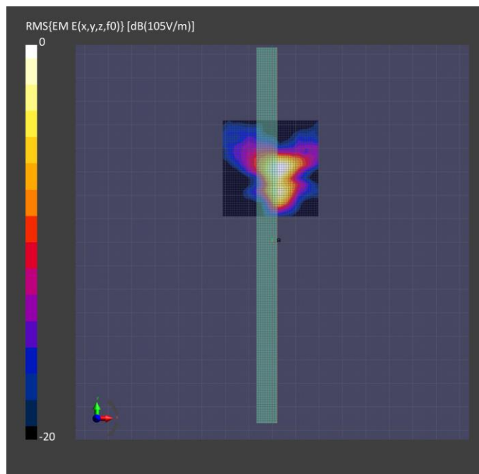
Figure 4-3: Band n261, beam ID 41, 4 cm 2 PD, Edge Right
