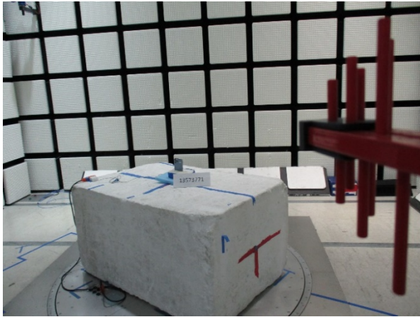
30 – 1000 MHz (FRONT)
