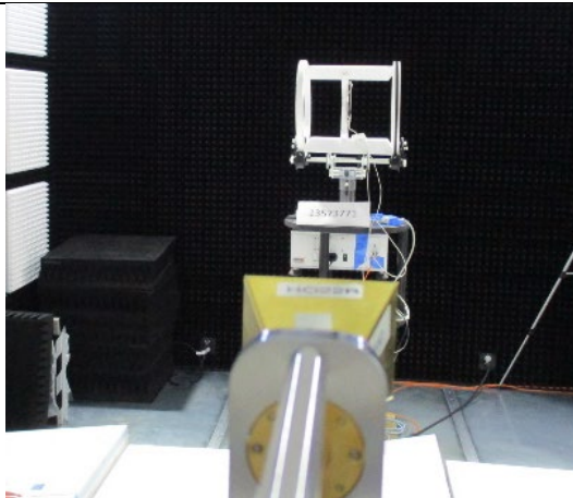
40 – 50 GHz (FRONT)
