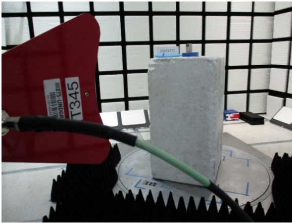
1 - 18 GHz (FRONT)
