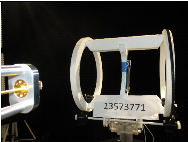
170 - 200 GHz (FRONT)
