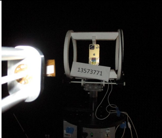
75 - 110 GHz (FRONT)
