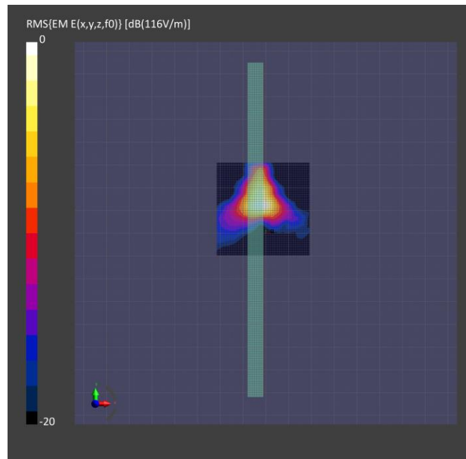
Figure 4-3: Band n261, beam ID 44/172, 4 cm 2 PD, Edge Right
