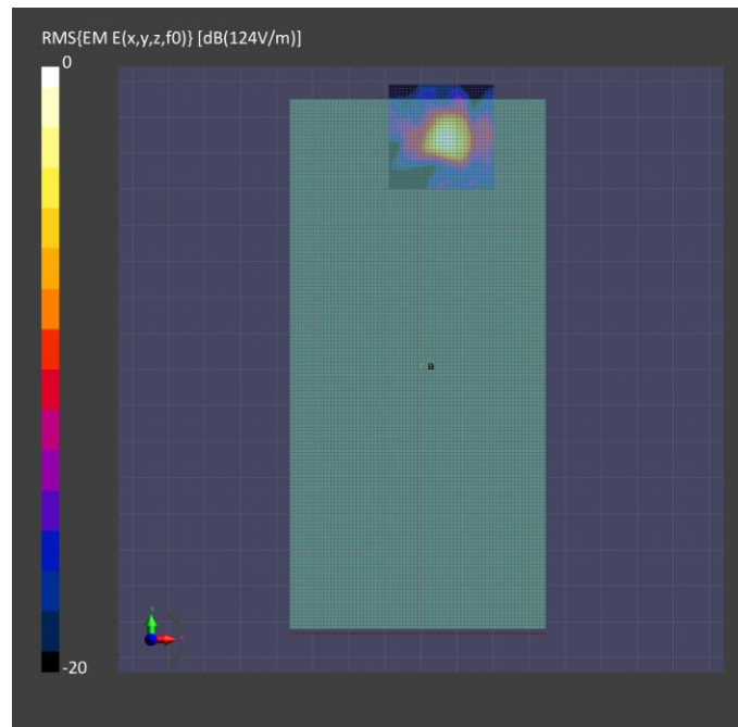
Figure 4-2: Band n260, beam ID 21, 4 cm 2 PD, Back
