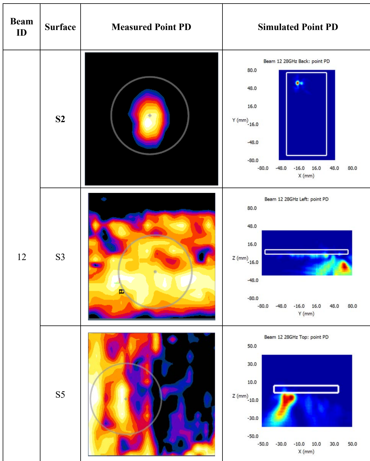
Figure 10. Simulated and measured point PD for different beams for n261.
