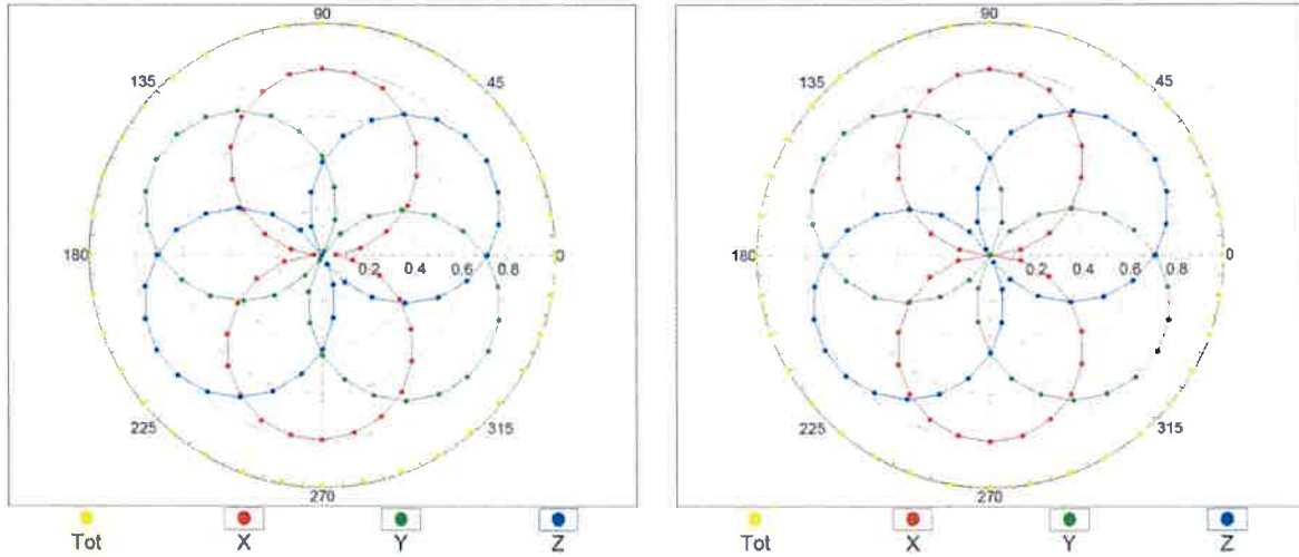
f=600 MHz,TEM
