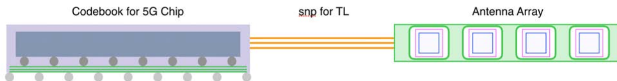
Figure 9. The process of excitation is from 5G chip to RF lines and to the antenna array
