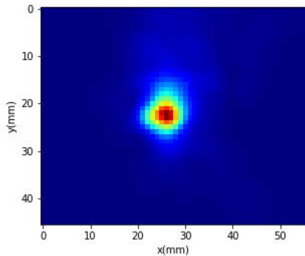
Power Density Plots for Beam ID:3
