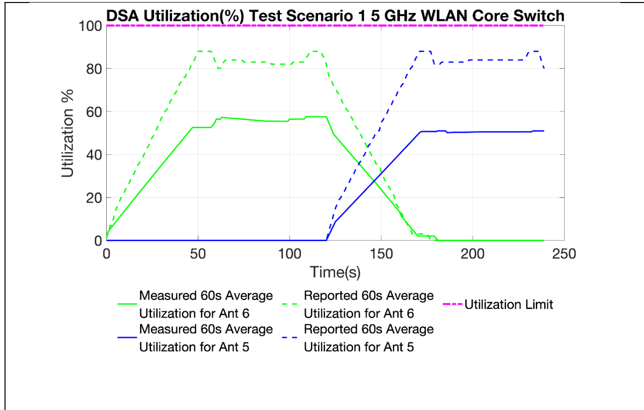
Figure 4 60 Second Aggregated SAR Utilization vs Time, 5GHz
