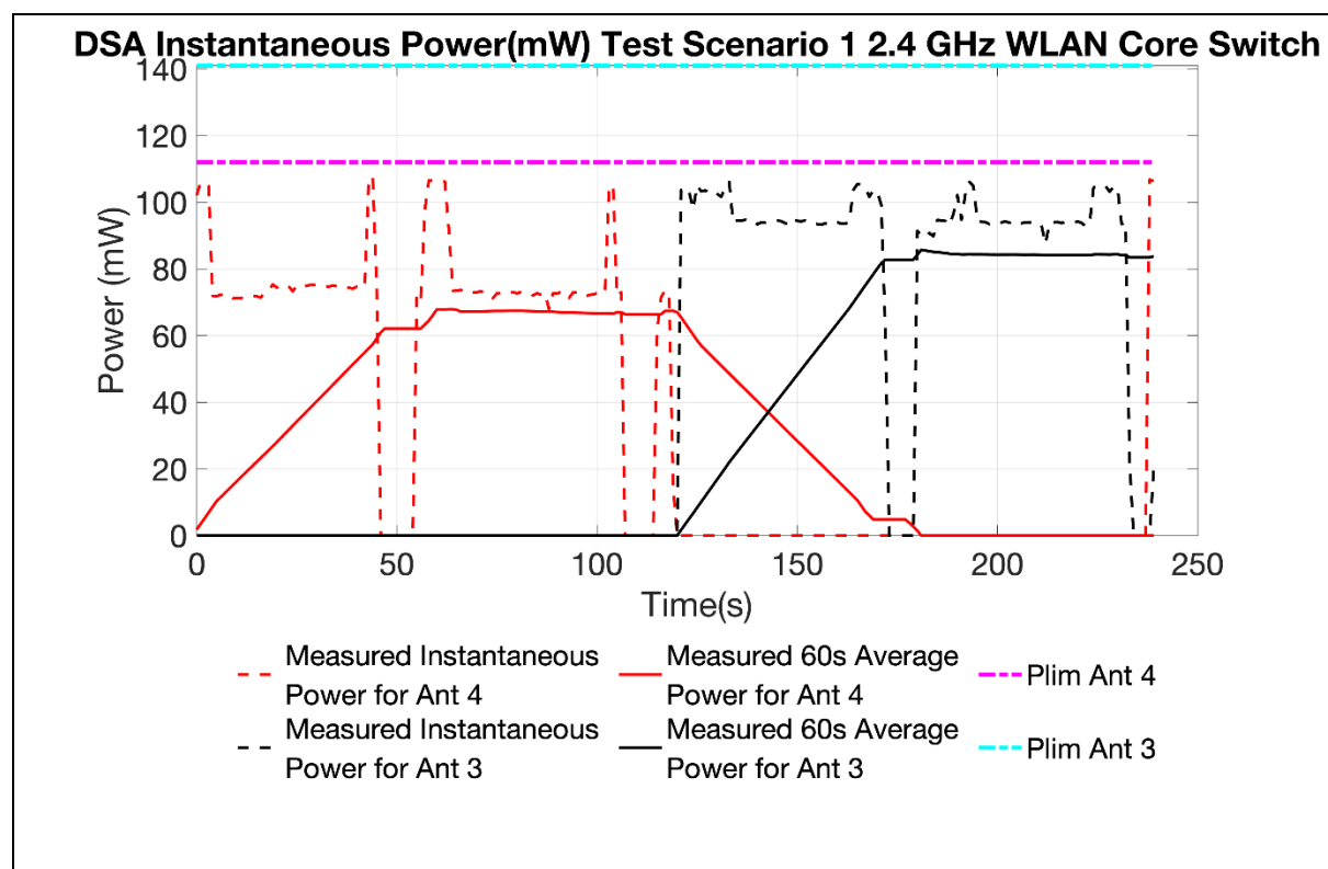
Figure 3 60 Second Average Power vs Time and Instantaneous Power, 2.4GHz
