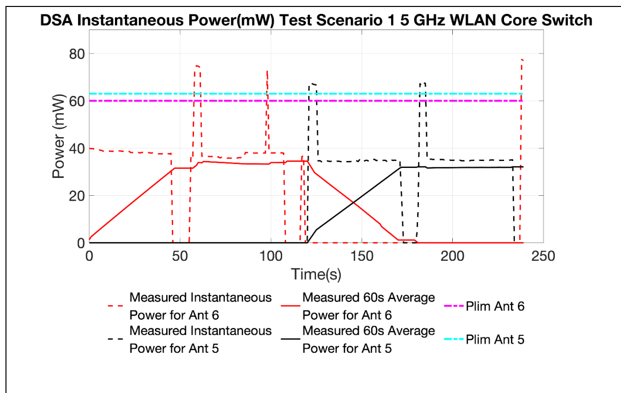
Figure 6 60 Second Average Power vs Time and Instantaneous Power, 5GHz
