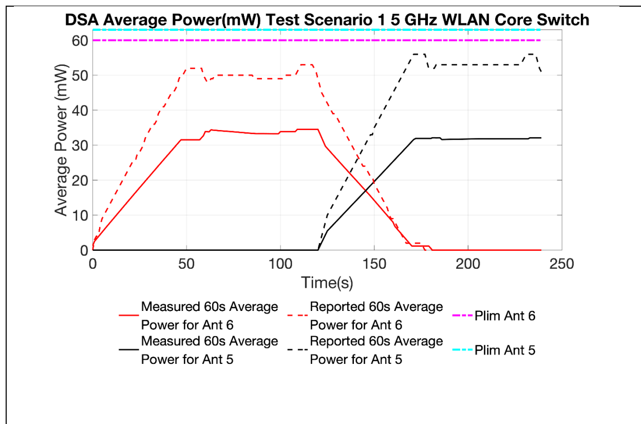
Figure 5 60 Second Average Power vs Time, 5GHz
