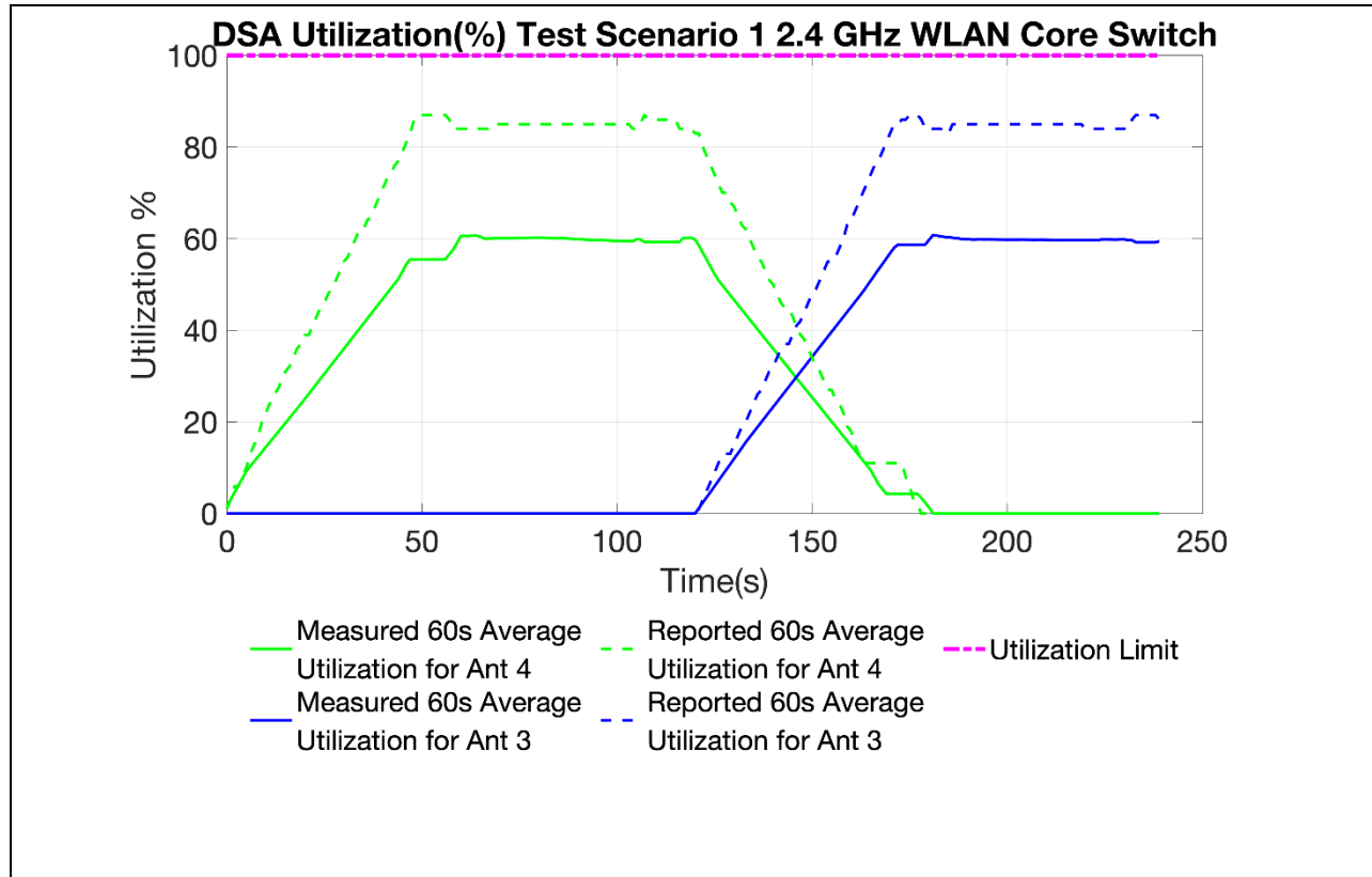
Figure 1 60 Second Aggregated SAR Utilization vs Time, 2.4GHz
