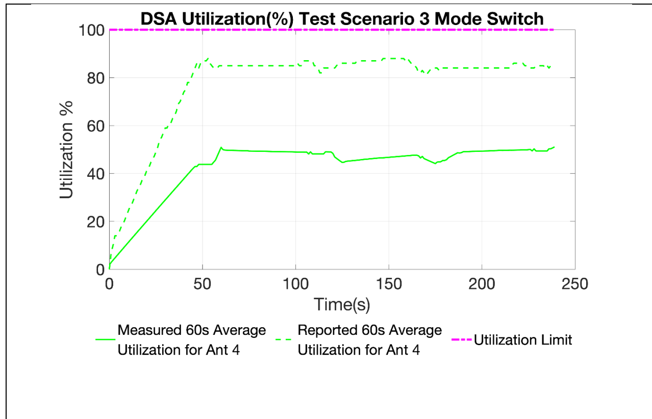
Figure 10 60 Second Aggregated SAR Utilization vs Time during Mode Switch
