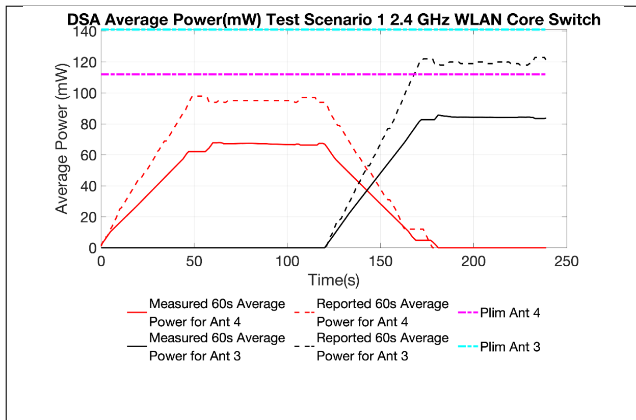
Figure 2 60 Second Average Power vs Time, 2.4GHz
