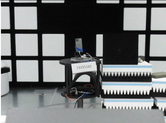
18 - 26 GHz (FRONT)
