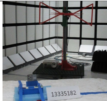
30 - 1000 MHz (BACK)
