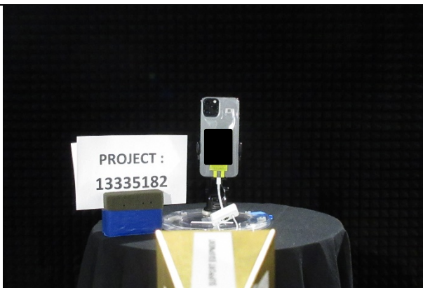
50 - 75 GHz (FRONT)
