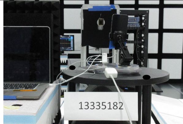
18 - 26 GHz (BACK)
