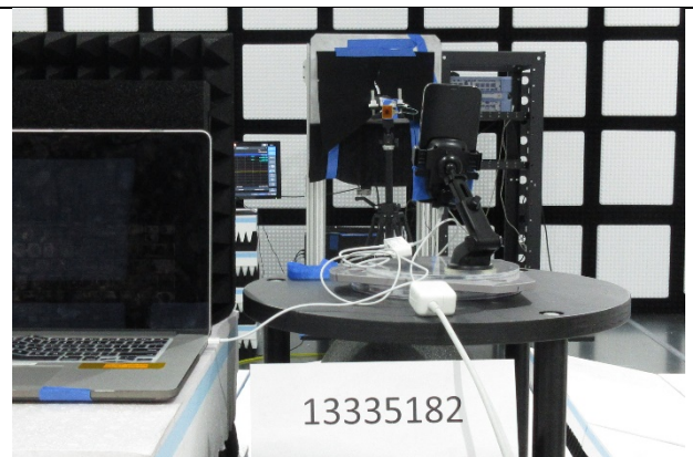
40 – 50 GHz (BACK)
