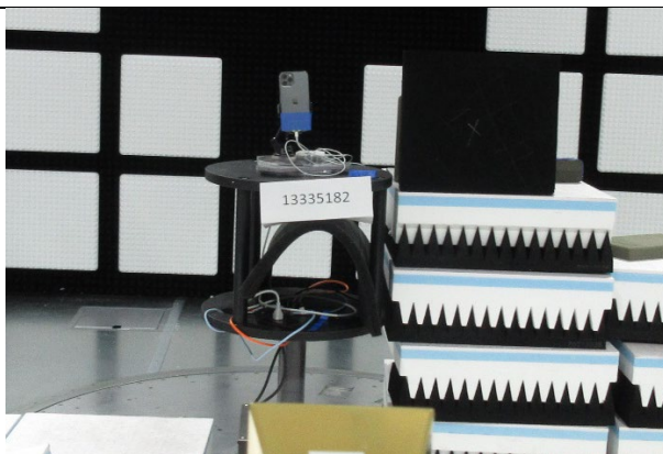
40 – 50 GHz (FRONT)
