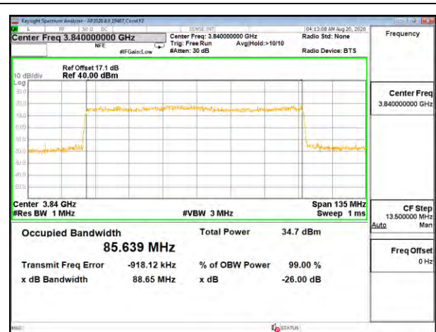
5G NR Band n77 90MHz QPSK Middle Channel RB240-0
