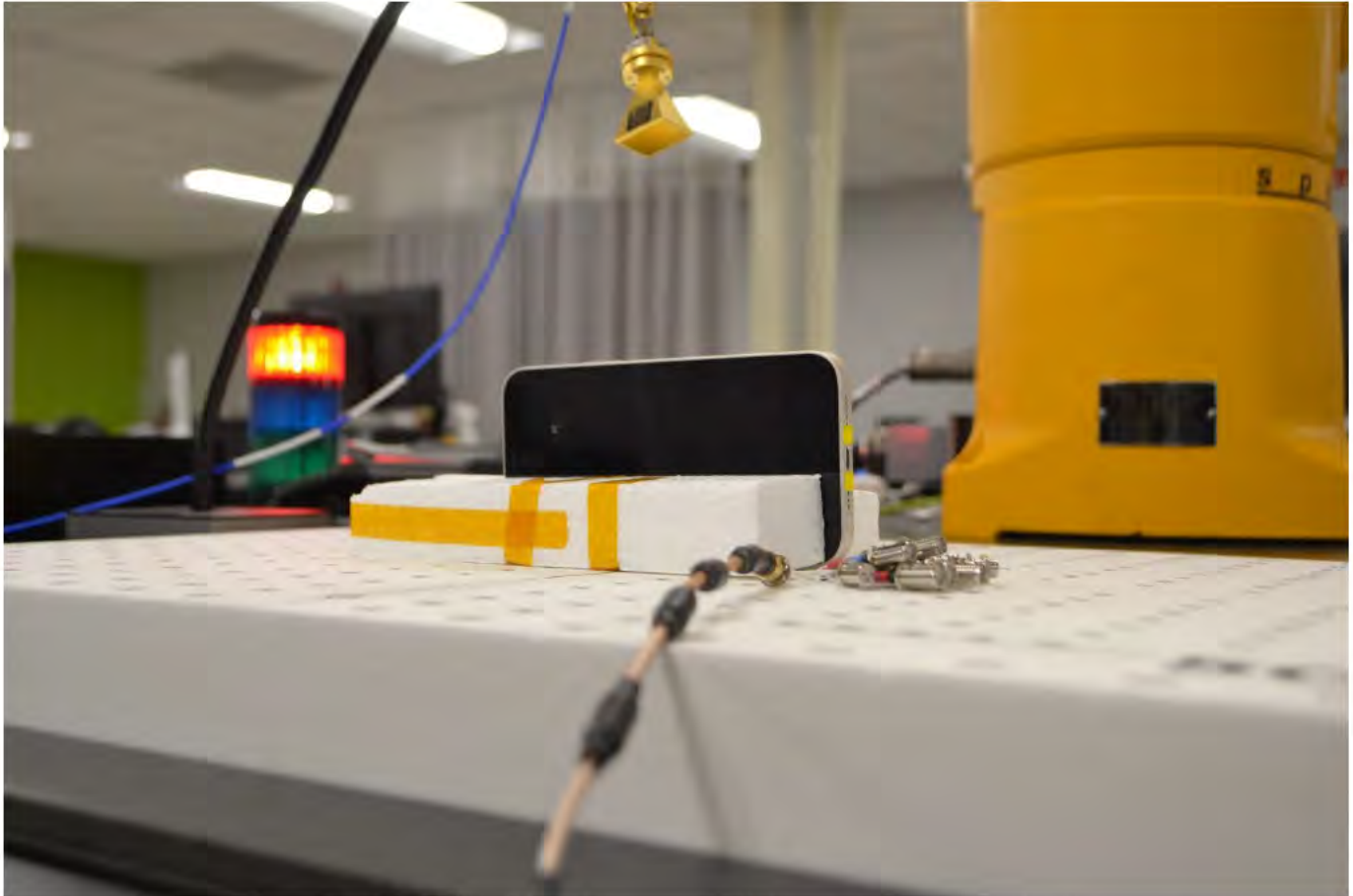
Figure C-4 DASY radiated power mmW test measurement setup
