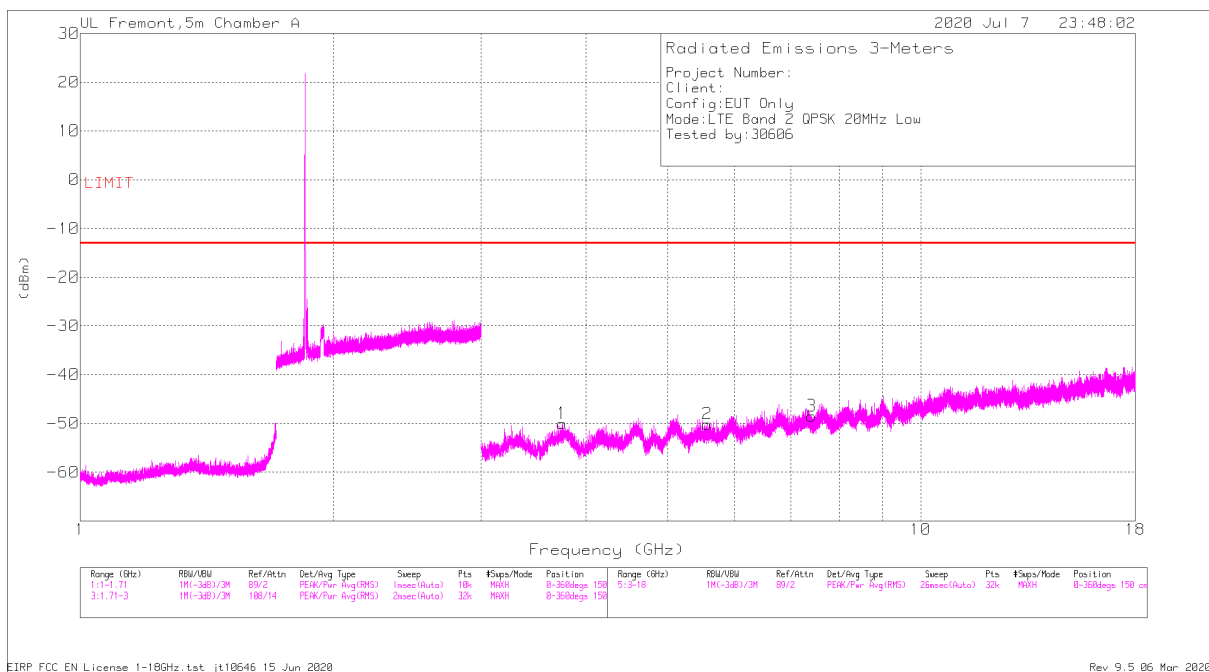
Horizontal Polarity
