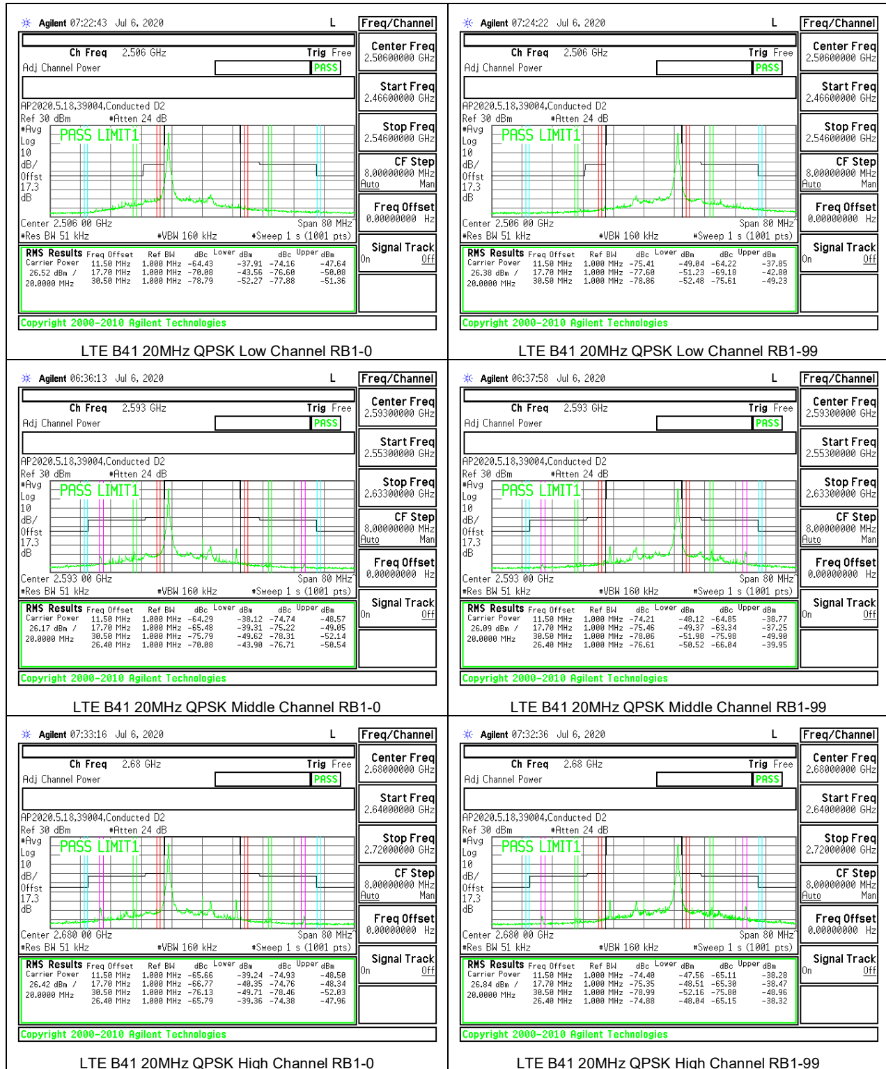
LTE B41 20MHz QPSK High Channel RB1-0
